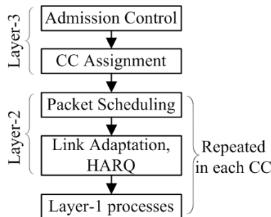
Fig. 1.2: Radio resource management in a multi-CC LTE-Advanced system.
