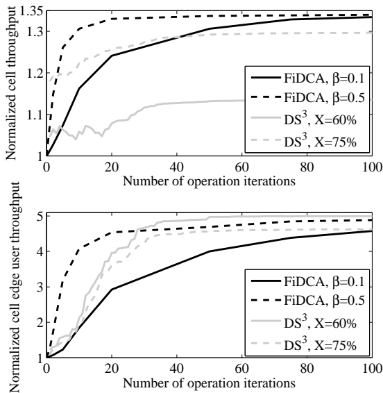
Fig. 3.20: Convergence time for FiDCA and DS 3 in the downlink of a 16-cell home scenario. All APs are activated.
