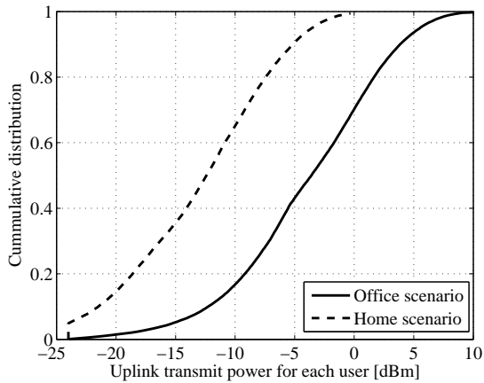
Fig. 2.3: CDF of uplink transmit power in home and office scenarios.
