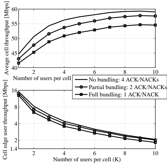
Fig. 5.12: Downlink throughput with ACK/NACK bundling and full buffer model.
