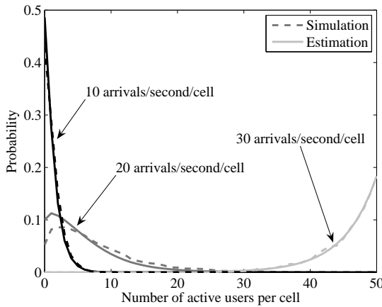
Fig. C.3: Probability of a cell being in different states of a Markov chain.
