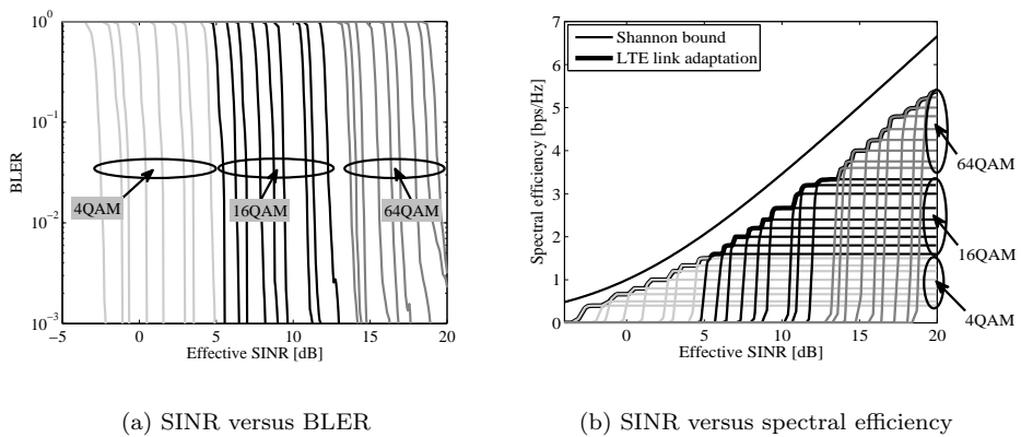
Fig. A.7: Mapping from SINR to BLER and spectral efficiency.
