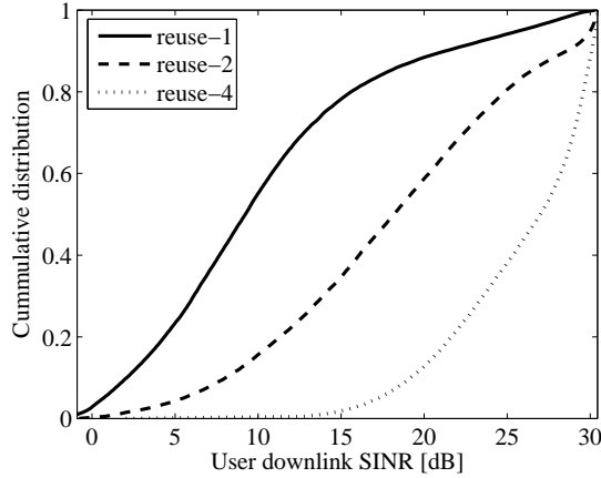
Fig. 3.8: CDF of downlink SINR with frequency reuse in the Manhattan scenario.
