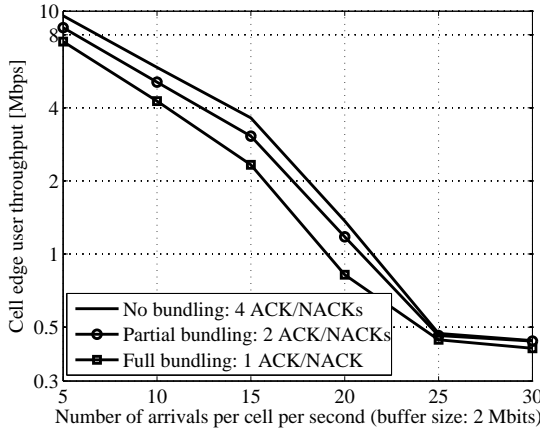
Fig. 5.13: Cell edge user throughput with ACK/NACK bundling. Finite buffer model is used with different arrival rates.
