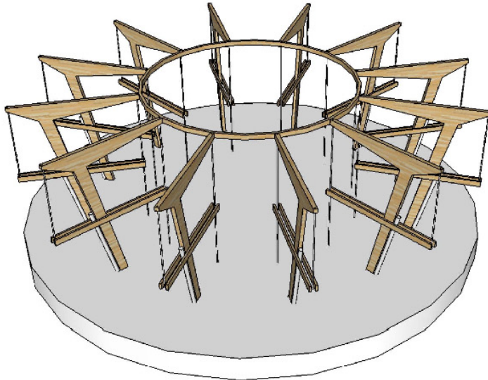
Figure 2.13. Laminated wooden elements form the main structural concept [illustration credit: Rudy Uytenga Architects]
