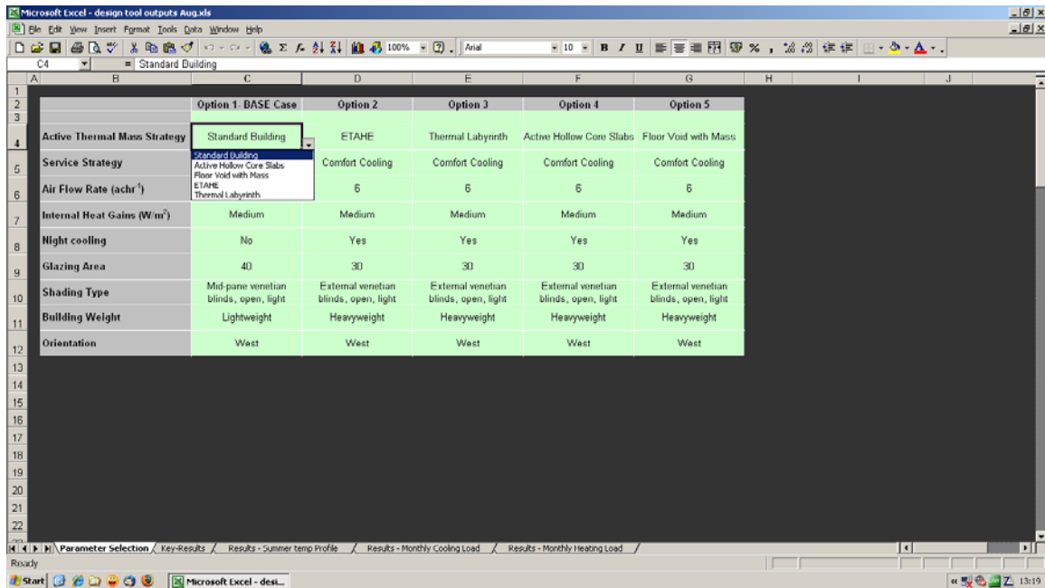
Figure 4.4 Opening tab of the concept design tool TMAir where the input parameter selection can be made.
