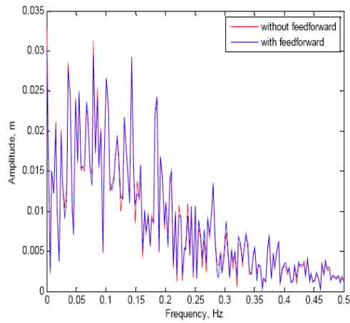
Figure 5.13: Single-Sided Amplitude Spectrum of y
