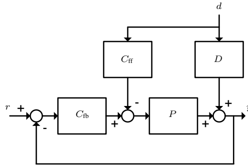
Figure 5.1: Feedforward control
