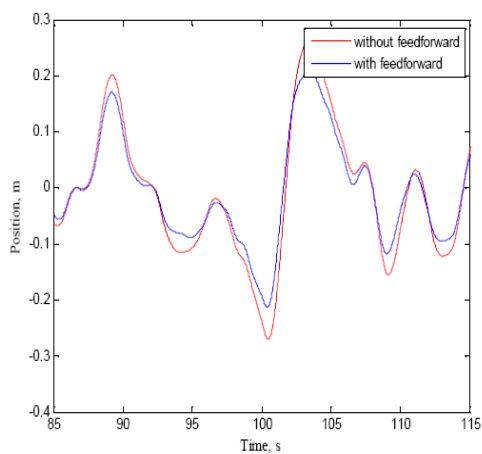
Figure 5.10: Position in x -axis, x . Imp = 17\%
