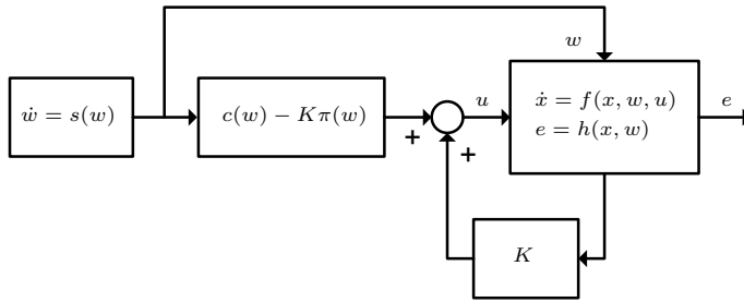
Figure 1.2: State feedback with feedforward control law
