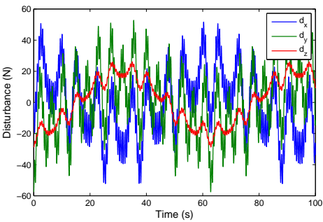
Figure 8.1: Wind disturbance
