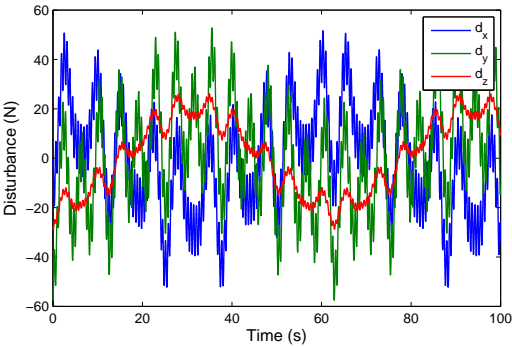
Figure 10.2: Wind disturbance
