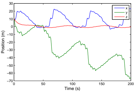
Figure 8.2: Position when disturbance adaptation is turned off.
