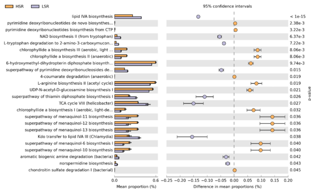
Fig. 8 Predictive metagenome functions that discriminate between pond microbiomes with different survival rates. HSR is grow-out ponds with a high survival rate and LSR is grow-out ponds with a low survival rate. Extended error bar plot for two-group analysis module comparison of PICRUSt predicted KEGG function data based on the HSR and LSR using Welch's t -test for the two groups.
