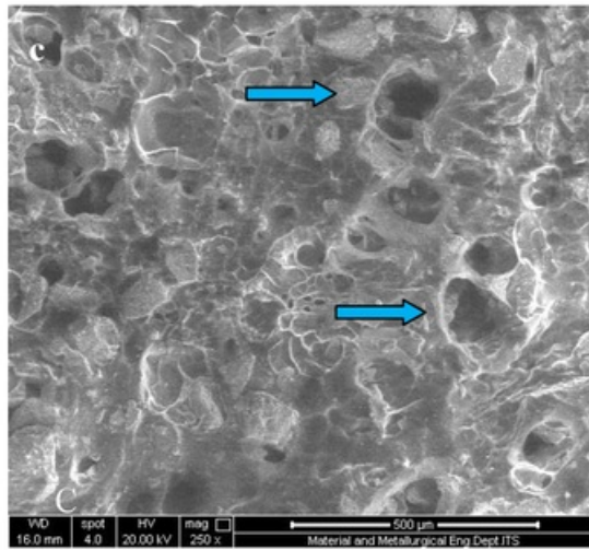
Figure 2. (a) Results of SEM test and porosity measurement test at the magnification of 75x; (b)100x; and (c) 250x.
