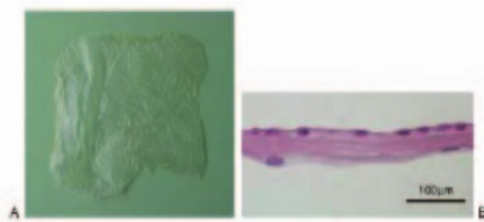
Fig. 1, Amniotic Membran (Tomita T, 2012)
