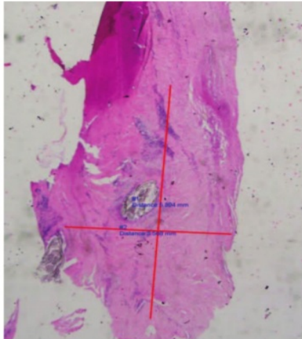
Fig 3. PA microscopic histological examination display with HE staining 40x magnification. Sample, obtained 5.89 mm x 3.57 mm fibrocytes infiltration.
