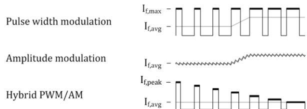
Fig. 3. Concept of different LED dimming schemes. I_{f,max} is the maximum forward current of an LED. Under PWM, the average current is controlled by the duty cycle. Under AM the average current is a directly controlled variable. Hybrid PWM/AM uses variable peak current and variable duty cycle to control the average forward current. Different combinations of peak current and duty cycle can be used to obtain the same value of the average current.
