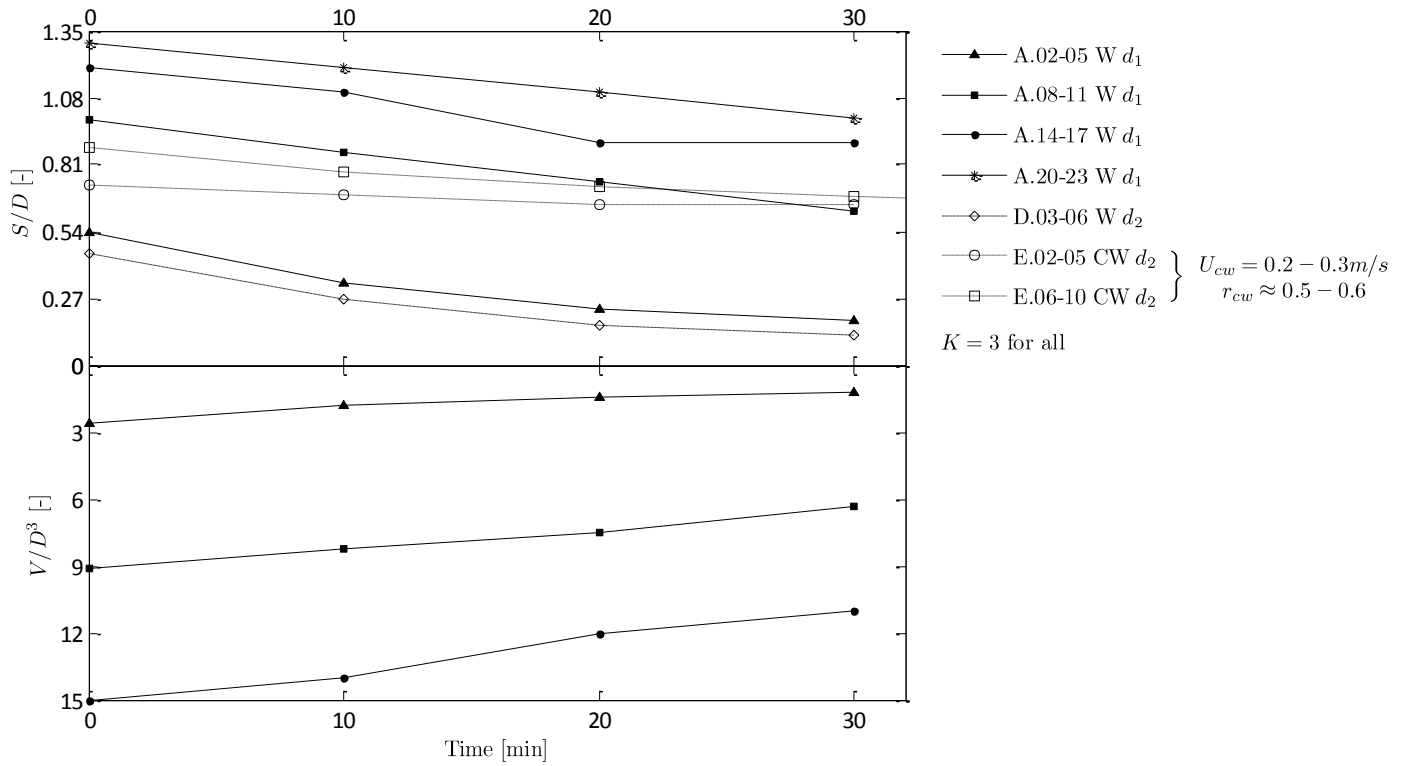
Figure 19: Normalized scour depth and normalized scour volume. Backfilling tests. Wave-only (W) flows or combined current and waves (CW). Grain sizes d_1 = 0.15mm or d_2 = 0.10mm .
