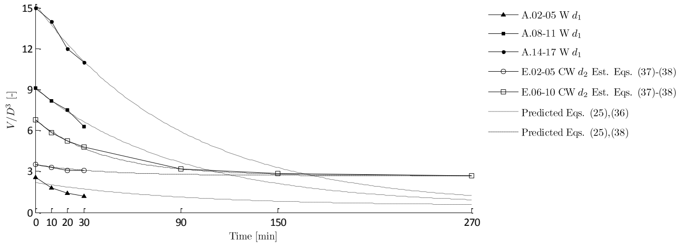
Figure 20: Measured and predicted normalized scour volume. Backfilling tests. Wave-only (W) flows or combined current and waves (CW). Grain sizes d_1 = 0.15mm or d_2 = 0.10mm .
