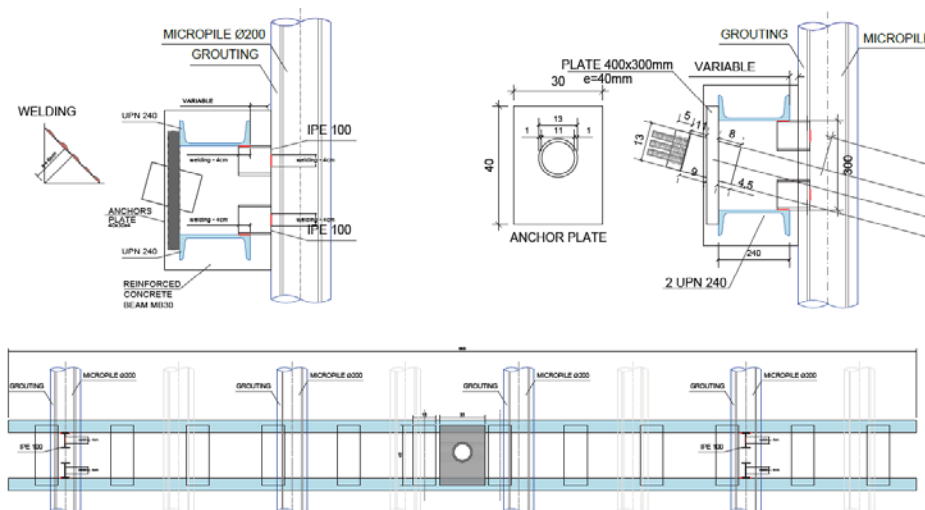
Figure 2. Detail steel beams and plates for anchors
