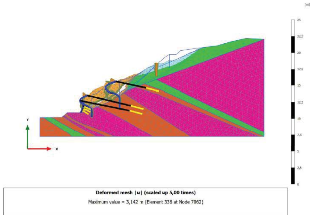
Figure 3. Deformed mesh for the cross section 878+800
