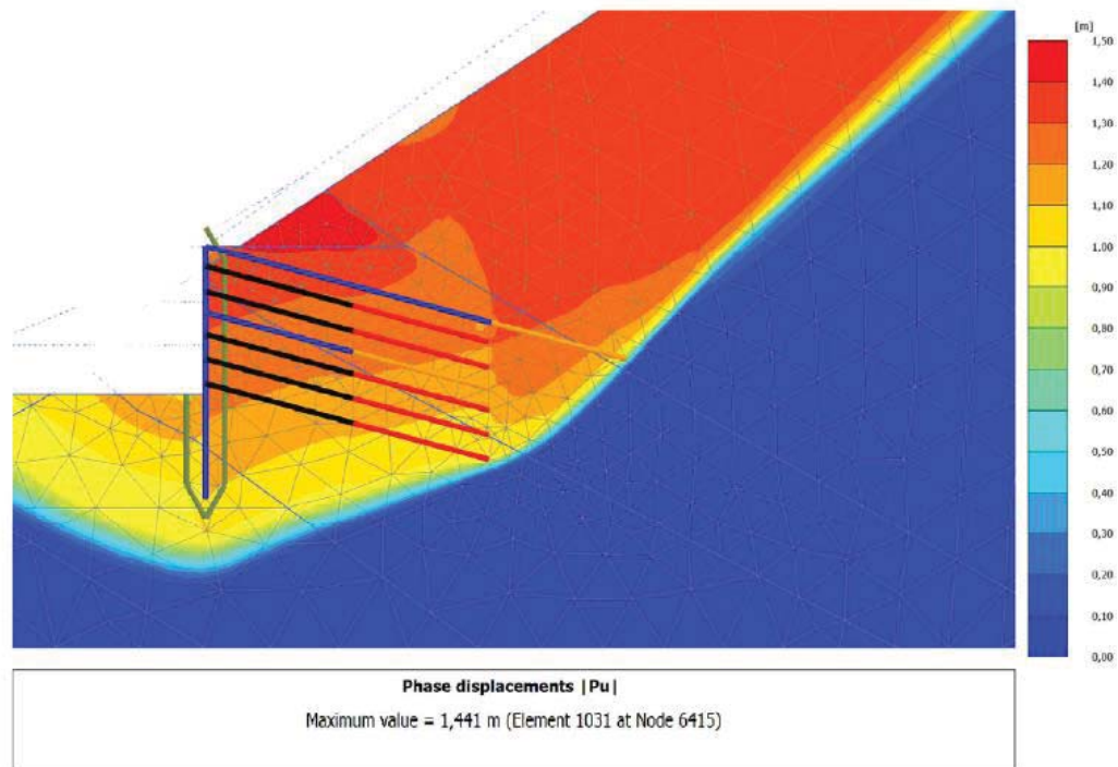
Figure 4. Deformed mesh for the cross section 878+950
