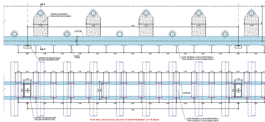
Figure 1. Plan and longitudinal section of tie beam
