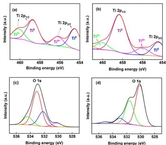
Figure 3: Deconvoluted XPS spectra of the titanium electrode (a) Ti 2p spectra before electrolysis, (b) Ti 2p spectra after electrolysis, (c) O 1s spectra before electrolysis, and (d) O 1s spectra after electrolysis.
