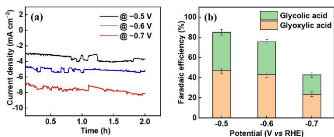
Figure 2: (a) the current densities of titanium electrodes at three different applied potentials ( -0.5 V, -0.6 V and -0.7 V vs RHE) and (b) the average Faradaic efficiency for production of glyoxylic and glycolic acids during bulk electrolysis of 0.03 M oxalic acid for 2 hours, using Ti foil as a working electrode and Pt foil as a counter electrode in an H-cell at 25 °C.
