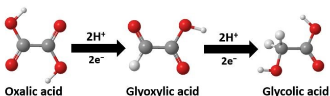
Figure 1: A pathway showing the reduction of oxalic acid to glyoxylic acid and glycolic acid. Colour code: white = hydrogen, red = oxygen, grey = carbon.
