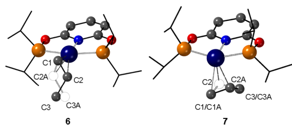
Figure 4. Comparison of structures of complexes 6 and 7 orientated to compare the propene coordination and disorder. [\text{BAR}_4^{\text{F}}]^- anions are not shown.
