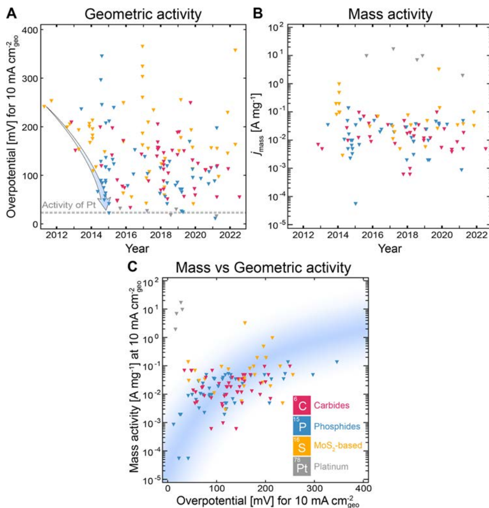
Figure 18. (A) Chronological trend in overpotential for a geometric current density of 10 mA cm -2 geo of carbide, phosphide and MoS 2 -based HER catalysts assessed in acidic electrolyte. Pt-based HER catalysts are shown for comparison; the dashed line is the average value of the data points. Blue arrow to guide the eye. (B) Chronological trend in the mass activity (evaluated at j = 10 mA cm -2 geo ) of the catalysts in (A). (C) Correlation of the mass activity in B and geometric activity in A. Shading to guide the eye. The data used in this figure and associated references are provided in the Supporting Information .
