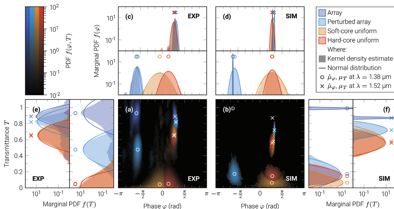
Figure 5. Probability density functions (PDFs) of transmittance and phase profiles. a, b) The maximum \max_{\tau, \lambda} f_{\tau, \lambda}(\varphi, T) of the PDFs f_{\tau, \lambda} of all metasurface types \tau (encoded by different colors) for the overlapping resonance case with resonant ( \lambda = 1.38 \mu\text{m} ) and off-resonant ( \lambda = 1.52 \mu\text{m} ) excitation (encoded by different marks) by a TE-polarized plane wave under normal incidence. c–f) Marginal PDFs, that is, integrals of f_{\tau, \lambda}(\varphi, T) along \varphi or T , where shaded areas result from kernel density estimates and solid lines show wrapped (c,d) and folded (e,f) normal distributions with matching means and variances. a, c, e) Experimental (EXP) and b, d, f) simulated (SIM) data.
