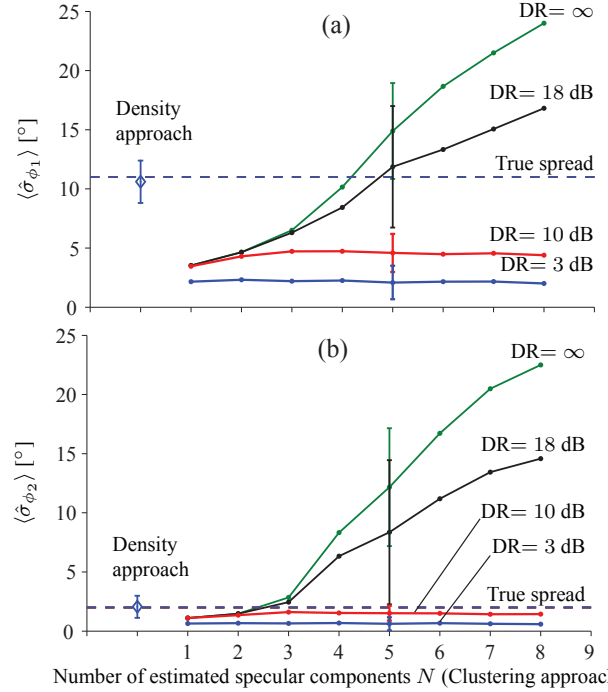
Fig. 3. Comparison of the estimated AoD spread (a) and AoA spread (b) computed with the density estimator and the clustering method. The clustering method uses different settings of the number of specular components N and DR. The error bars indicate the standard deviations of the estimates.
