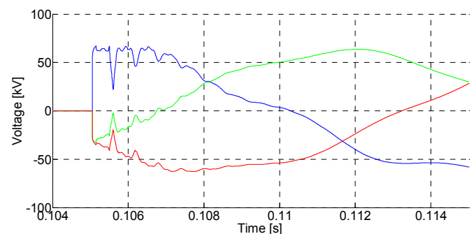
Fig. 13. Voltage in the open end of cable B41 during its energization using an equivalent network (Blue: Phase A, Green: Phase B, Red: Phase C)
