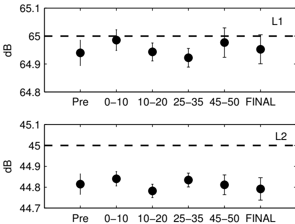
FIG. 8. Stability of the overall primary levels L1 and L2 at different intervals. The errorbars show the confidence interval ( \alpha = .05 ). The dashed horizontal lines show target levels of 65 and 45 dB.
