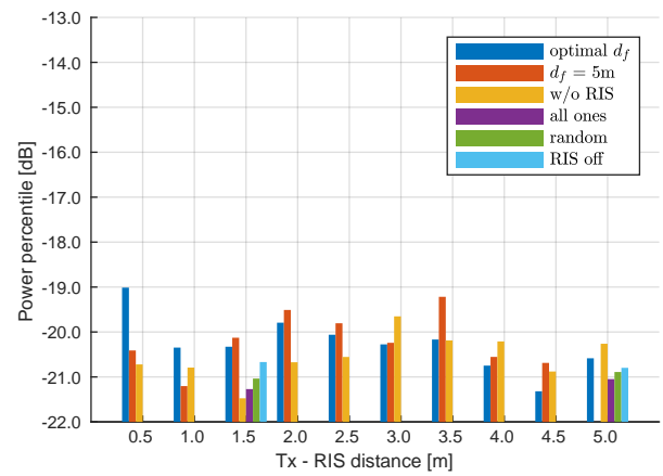
(a) Vertical Tx polarization
