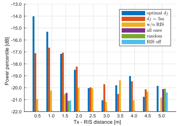
(b) Horizontal Tx polarization
