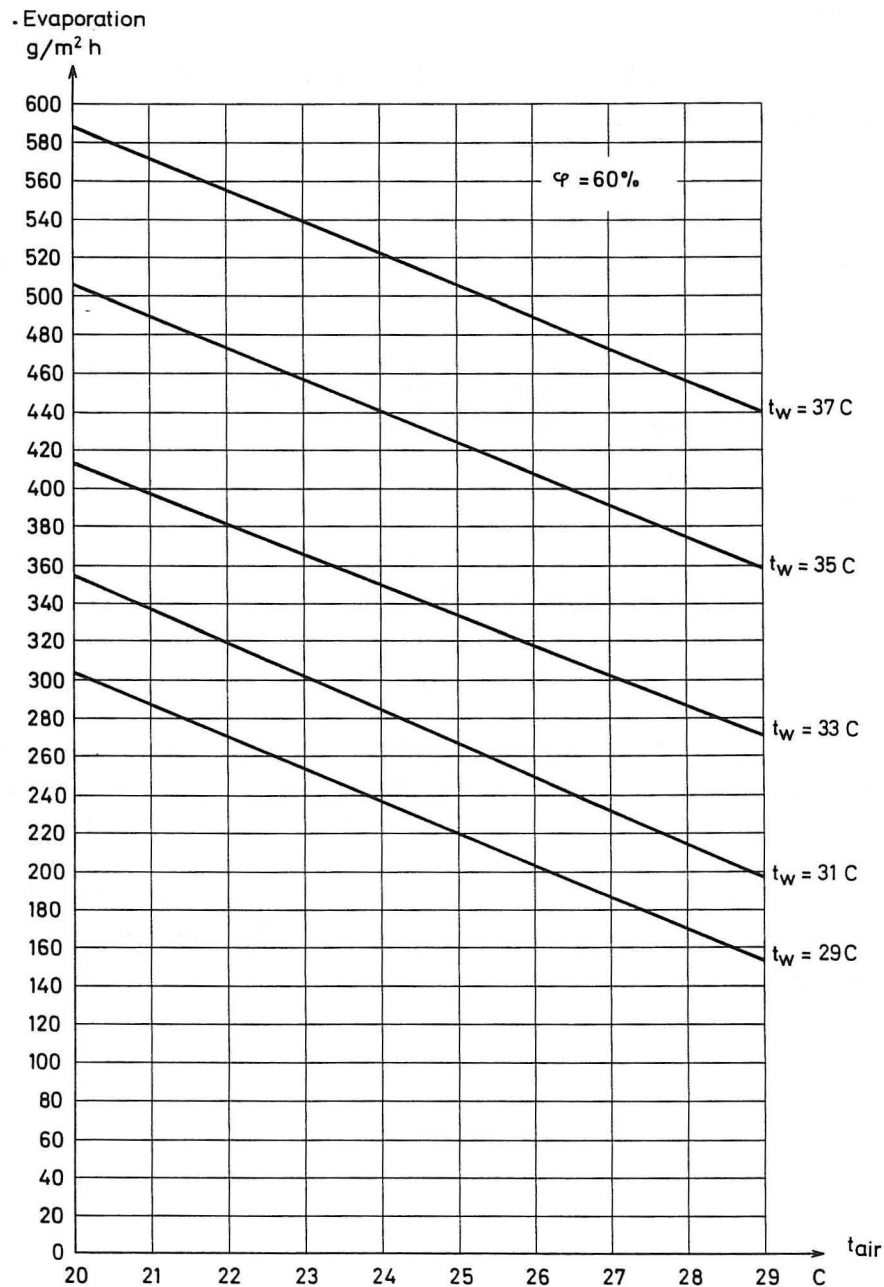
Fig. 11. Evaporation from a quiet water surface. The air temperature t_{air} and humidity \phi are measured 20 cm above the surface. The water surface temperature is t_w . The mean air velocity measured 2 cm above the surface is v = 0.15 m/s. Warning: you can interpolate but not extrapolate in the graphs.
