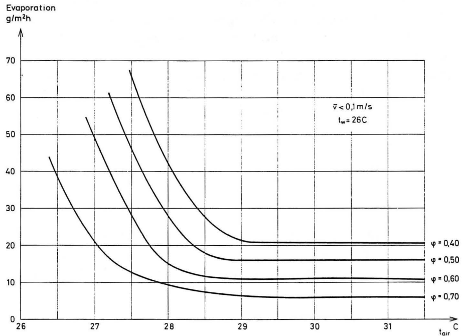
Fig. 5. Evaporation from a quiet surface of water. The air temperature t_{air} and humidity \phi are measured 20 cm above the surface. The water surface temperature is t_w . The mean air velocity v is measured 2 cm above the surface. Warning: you can interpolate but not extrapolate in the graph!
