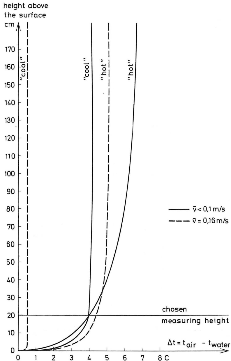
Fig. 2. Temperature in the air above the centre of the basin. Air velocity 2 cm above the surface = \bar{v} . Water temperatures between 24 and 28 C.
