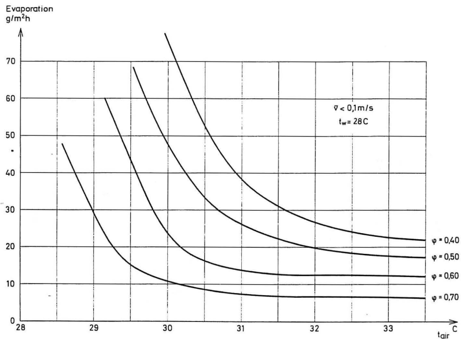
Fig. 6. Evaporation from a quiet surface of water. The air temperature t_{air} and humidity \phi are measured 20 cm above the surface. The water surface temperature is t_w . The mean air velocity v is measured 2 cm above the surface. Warning: you can interpolate but not extrapolate in the graph!
