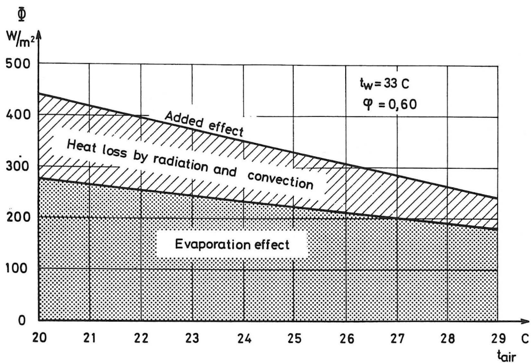
Fig. 14. Water heat balance at 33 C.
