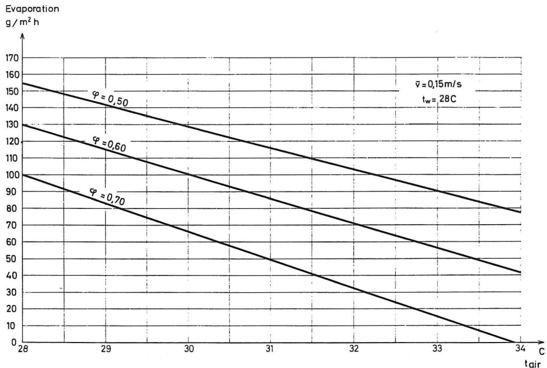
Fig. 8. Evaporation from a quiet surface of water. The air temperature t_{air} and humidity \phi are measured 20 cm above the surface. The water surface temperature is t_w . The mean air velocity v is measured 2 cm above the surface. Warning: you can interpolate but not extrapolate in the graph!
