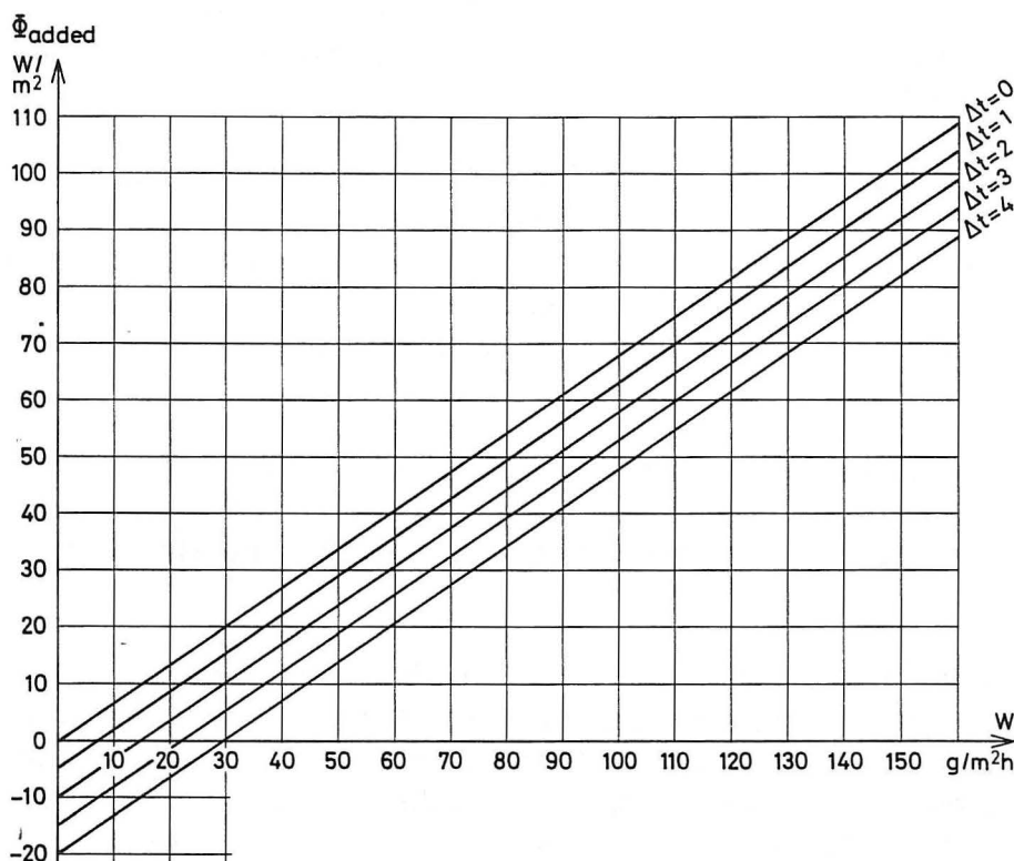
Fig. 9. Necessary heating added to the basin water \Phi_{\text{added}} as a function of the evaporation W . \Delta t = t_{\text{air}} - t_{\text{w}} is parameter. Air velocity 2 cm above the surface = 0.15 m/s.
