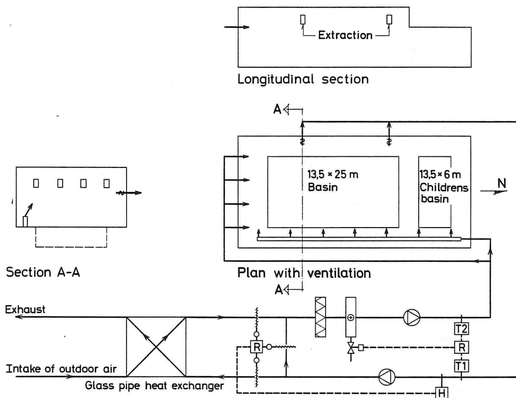
Fig. 17. Ventilation plan for Aars swimming bath. The flow of fresh air is controlled by the humidity probe H placed in the extraction pipe. The temperature in the room is controlled by the thermostat T1 placed in the extraction pipe yet the minimum thermostat T2 is setting the lower limit to the inlet temperature.
