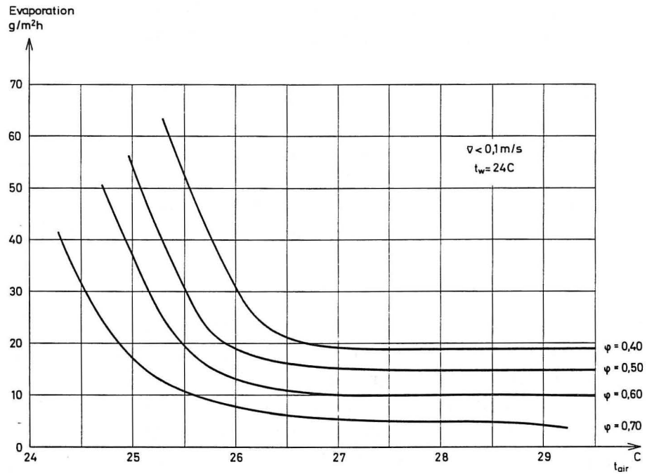
Fig. 4. Evaporation from a quiet surface of water. The air temperature t_{air} and humidity \phi are measured 20 cm above the surface. The water surface temperature is t_w . The mean air velocity v is measured 2 cm above the surface. Warning: you can interpolate but not extrapolate in the graph!
