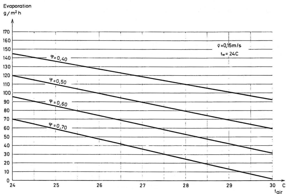
Fig. 7. Evaporation from a quiet surface of water. The air temperature t_{air} and humidity \phi are measured 20 cm above the surface. The water surface temperature is t_w . The mean air velocity v is measured 2 cm above the surface. Warning: you can interpolate but not extrapolate in the graph!
