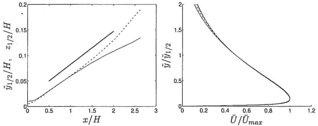
(a) Thin solid line: \bar{y}_{1/2} ; dashed line: z_{1/2} ; thick solid line: 0.065x .
