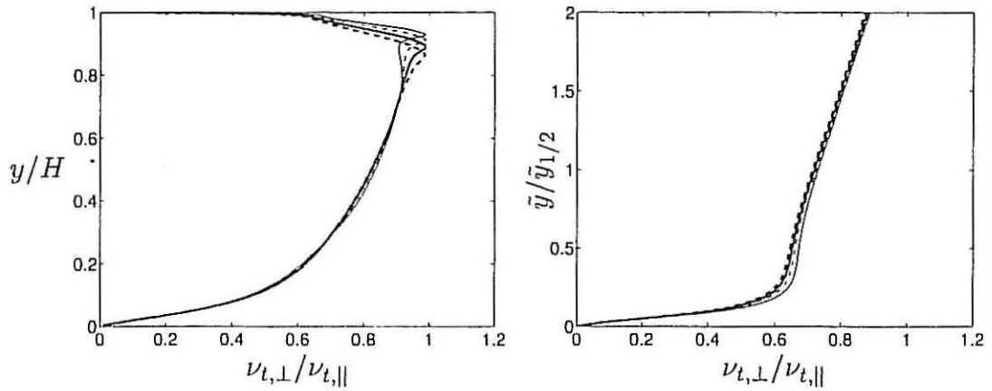
(a) Profiles between x/H = 0.34 and x/H = 1.07 .
