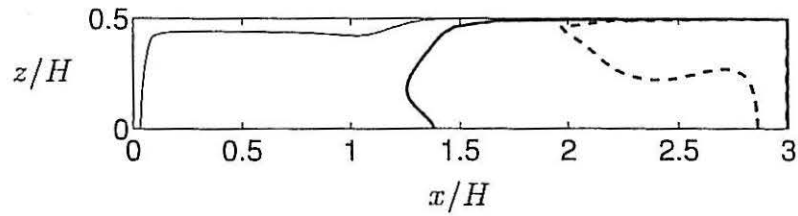
(a) Horizontal plane y/H = 0.2 .
