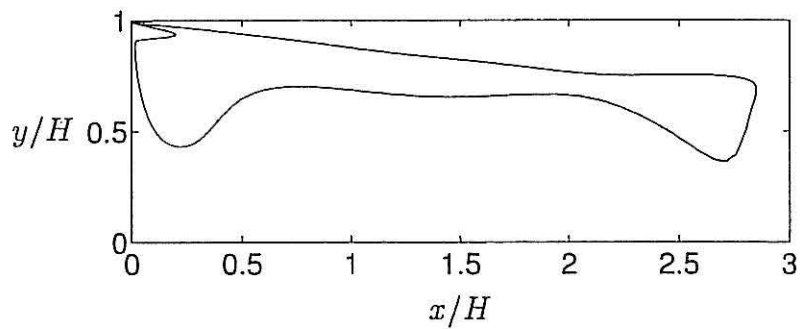
(c) \overline{v^2} - f model, Modification I. y/H = 0.98
