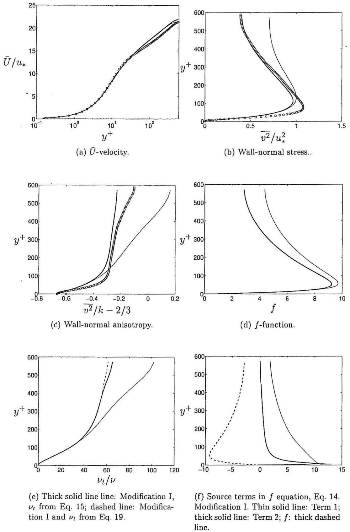
Figure 2: Channel flow. Re_\tau = 590 . \bar{v}^2 - f model. Thin solid line: standard model; thick solid lines: Modification I. Circles represent DNS of Moser et al. (1999)
