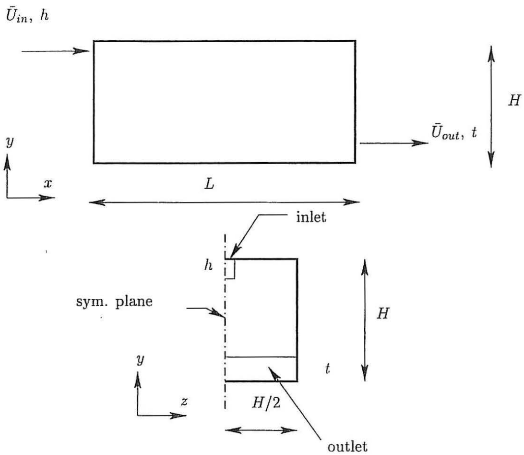
Figure 3: Configuration. L = 3H , h/H = 0.01 , t/H = 0.15 . Re = \bar{U}_{in}h/\nu = 7000 .
