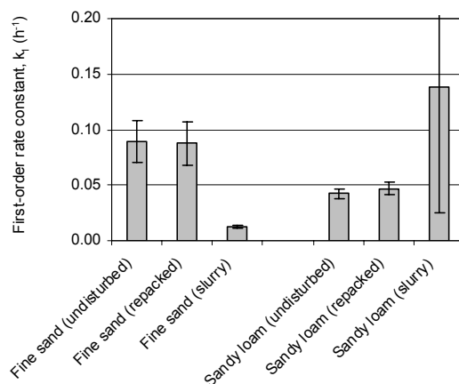
Figure 13. Mean first-order rate constants of benzene biodegradation determined for undisturbed soil cores, repacked soil cores, and soil slurries, respectively, using two sandy soils. Error bars correspond to the standard deviation. All soil cores were wetted to saturation in a sand box and drained to a water potential of -10 kPa.
