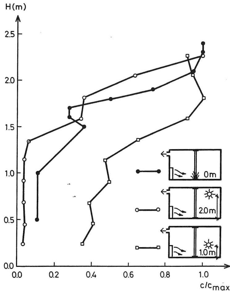
Figure 13. Normalized distribution of contamination in the room with release of tracer gas into the boundary layer flow and into the room 2.0 m and 1.0 m above floor, respectively.
