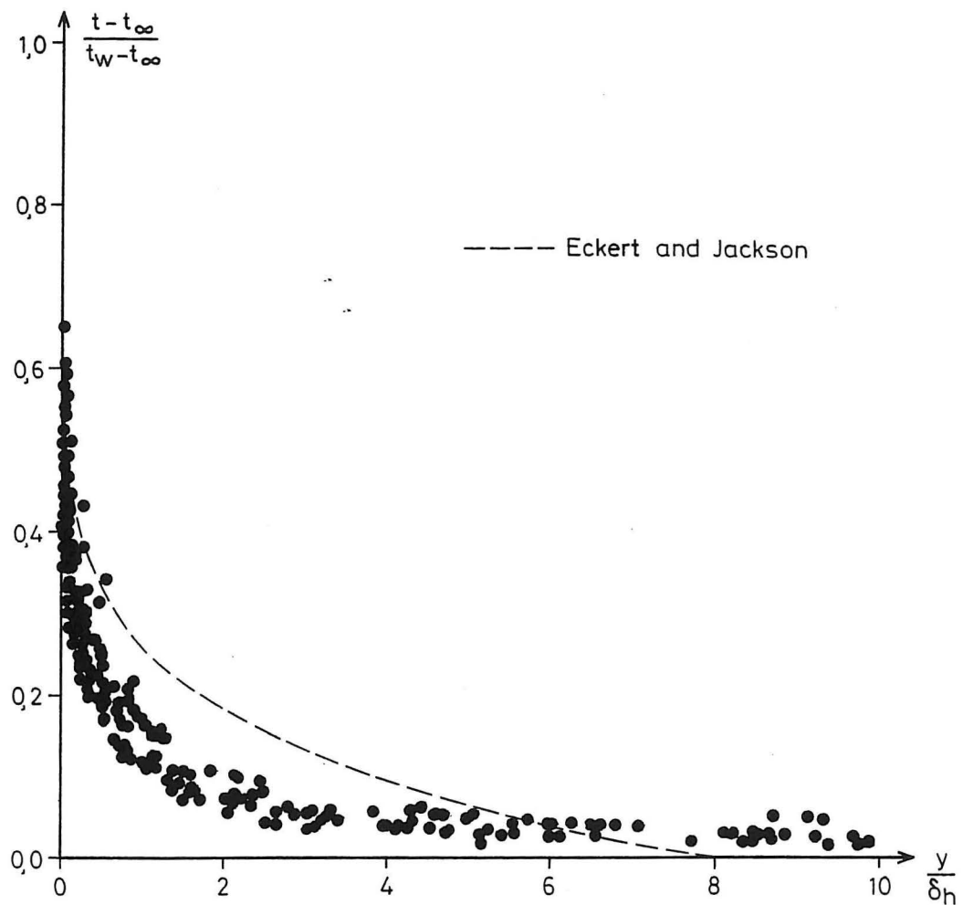
Figure 5. Recorded temperature distribution in the boundary layer.
