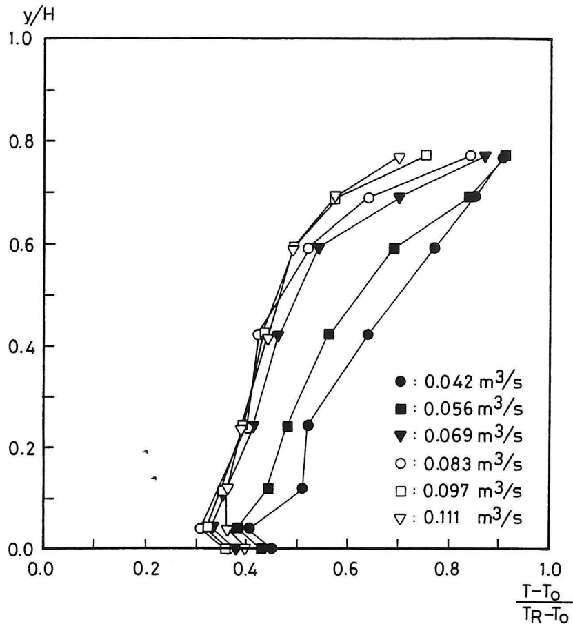
Fig. 10. Vertical temperature distribution for different air flow rates. Diffuser type B. Q = 500 W. Measurements by M. Andersen et al. 7 .
