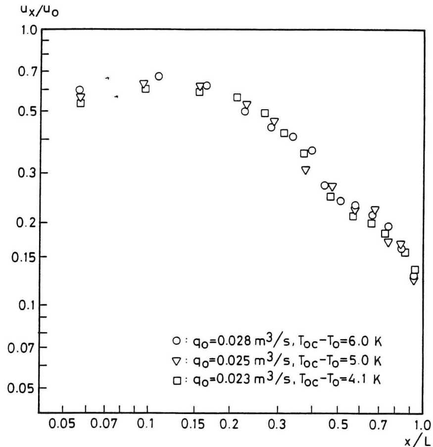
Fig. 7. Velocity decay versus distance measured for identical Archimedes number, for three different Reynolds numbers. Diffuser type B.
