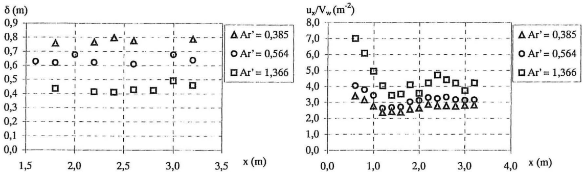
Figure 10: The width of the jet ( \delta ) and the relative velocity level versus the distance x . Shown for 3 different Ar^2 -numbers with an opening area of A_{win} = 0.089 \text{ m}^2 .
