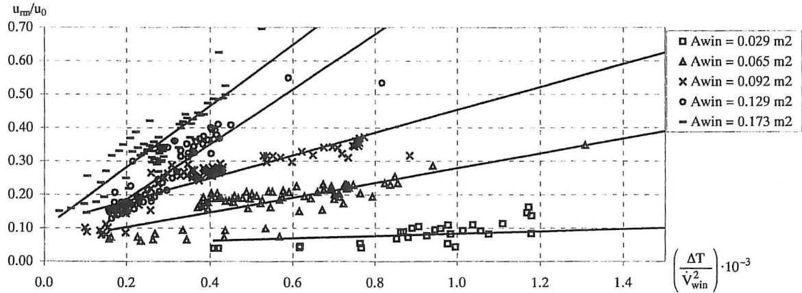
Figure 9: W1: Measurements of the maximum velocity in the occupied zone for 5 opening areas versus Ar^2 . Matching linear regression lines are shown for all 5 opening areas.
