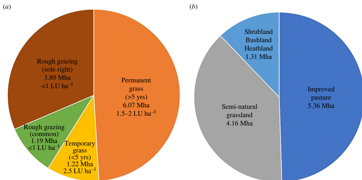
Figure 1. (a) UK agricultural area that is grassland or used for grazing, total 12.4 Mha (million hectares) (1). Typical stocking rates in livestock units per hectare (LU.ha -1 ) are also given, based on industry recommendations, where cattle over 2 years are 1 LU, and a lowland ewe with lamb is 0.12 LU. (b) UK land cover of habitat types that can be used for grazing (2).
