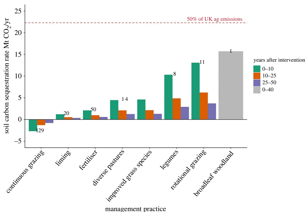
Figure 2. Carbon sequestration or emission rates from adopting grassland management practices, assumed to be adopted over 20% of UK improved pasture area from figure 1 b (i.e. 1.07 M ha). Positive values are carbon sequestration, negative values represent emissions. Average sequestration rates presented from years 0–10, 10–25 and 25–50 following intervention adoption, demonstrating the declining rates of sequestration/emissions over time as soil carbon stocks approach a new equilibrium. The numbers above each group of bars indicate the number of primary studies underpinning that data point. The red dashed line at 22.3 Mt CO 2 e/yr represents half (50%) of UK agriculture emissions in 2020 (total 44.6 Mt CO 2 e (3)), included as a point of reference.
