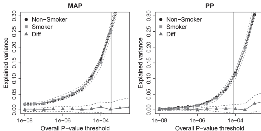
Figure 4. Smoking-specific estimates of variance explained in European ancestry. The variants with P \leq 5 \times 10^{-8} explained 1.9% of variance in MAP and 0.5% of variance in PP, whereas variants with P \leq 10^{-4} explained 16% of variance in MAP and 11% of variance in PP. The vertical line corresponds to FDR = 0.1.
