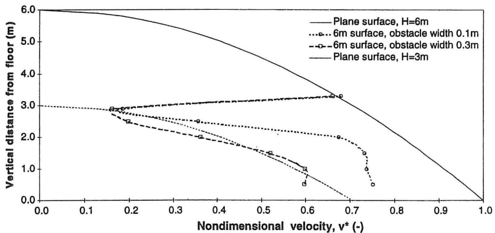
Figure 4 Non-dimensional maximum velocity in the boundary layer flow in different heights above the floor and for a temperature difference, \Delta t=9\text{K} . The values are measured at 6 m high surfaces with obstacles of different widths and calculated for plane surfaces of heights of 3 m and 6 m, respectively.
