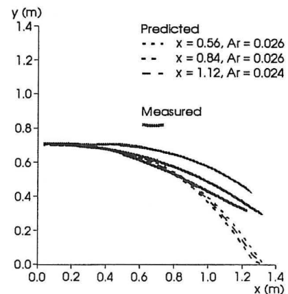
d: Comparison of measured and predicted pathway of supply air jet.
