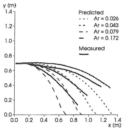
e: Comparison of measured and predicted pathway of supply air jet.
