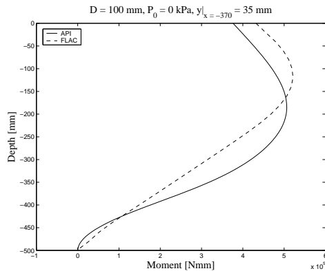
Figure 27: The moment curves obtained by means of the Winkler model approach with the ultimate soil resistance calculated by the design regulation formulation incorporated and the numerical model for D = 100 mm and P_0 = 0 kPa
