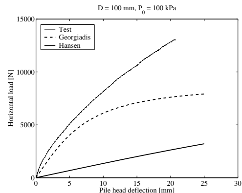
Figure 24: Load-deflection relationships measured at the level of the hydraulic piston ( x = -370 mm) obtained from the tests and the Winkler model approach with the two expressions for the ultimate soil resistance accounting for the overburden pressure incorporated. D = 100 mm. P_0 = 100 kPa. The initial modulus of subgrade reaction, k , is set to 40000 \text{kN/m}^3 .
