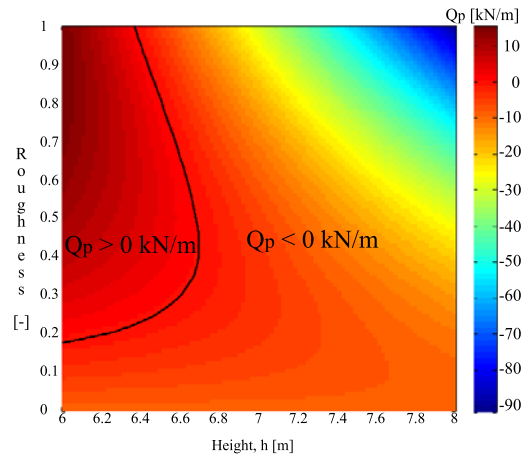
Figure 4: Parametric analyses of the point load Q_p at the pile toe as a function of the height and the roughness for a free sheet pile wall.
