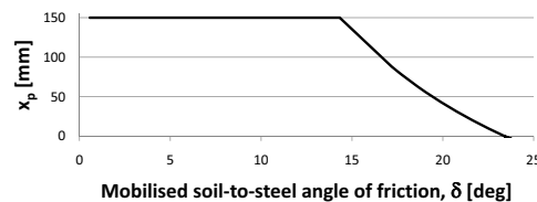
Figure 10: The plugged length x_p as a function of the mobilised soil-to-steel angle of angle of friction an H-section placed in Aalborg Clay.
