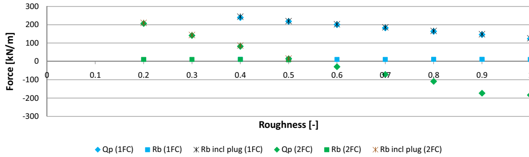
Figure 6: Parametric analysis on the roughness on a anchored sheet pile wall. Q_p is the force needed to be transferred to the soil to fulfil vertical equilibrium. R_b and R_b incl. plug is the base resistance of the steel and the plugged area, respectively.
