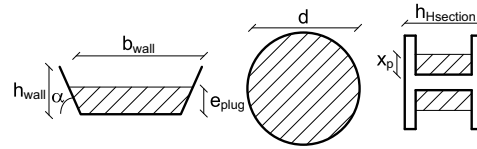
Figure 9: Sketch of the areas in which plugging occurs for different geometries.
