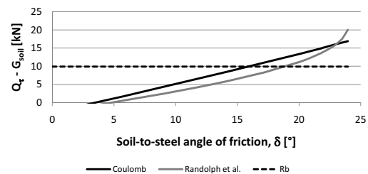
Figure 12: The skin friction reduced for soil weight and the static end bearing capacity as a function of the soil-to-steel angle of friction for the case study in Aalborg Clay.
