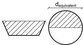
Figure 8: The equivalent diameter calculated by letting the hatched area of the sheet pile wall being equal to the hatched area of the circle.
