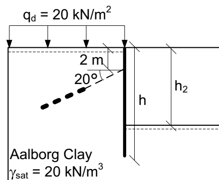
Figure 3: Sketch of the geometry used when calculating the vertical equilibrium of sheet pile walls.
