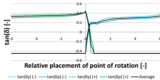
Figure 5: Difference between \tan \delta_\gamma and \tan \delta_p for a perfectly rough wall.
