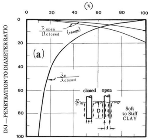
Figure 7: The effect of a plug upon the static bearing capacity. After Paikowsky and Whitman (1990).
