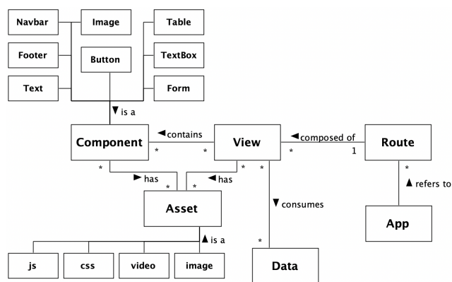
Fig. 5. Vue.js component architecture meta-model.
