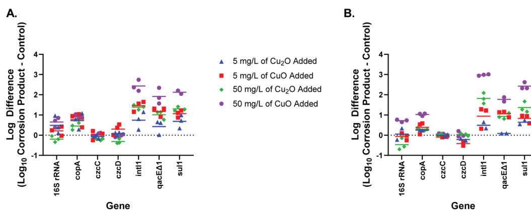
Fig. 3 Log difference in gene counts, measured with qPCR, between corrosion product conditions vs. the no addition control on (A) day 3 and (B) day 7. Copper corrosion product type and concentration added on day 0 to each microcosm are indicated by the color–symbol combination. Genes quantified: 16S rRNA = total bacteria, copA , czcC , and czcD = metal resistances, intI1 = integron-integrase known to carry resistances, qacEΔ1 = antiseptic resistance, and sul1 = antibiotic, sulfonamide resistance. For all graphs, points above the dashed line indicate more gene abundance than in the control, while points below dashed line indicate gene abundance was less than in the control. The statistical significance of each of the scenarios shown is indicated in Fig. 5.
