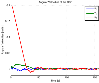
(a) Truth model angular velocities
