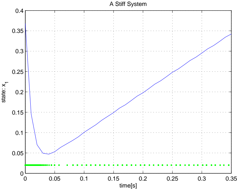
Figure 3.7: Example of a system with different response time-scales and the resulting internal integrator events.
