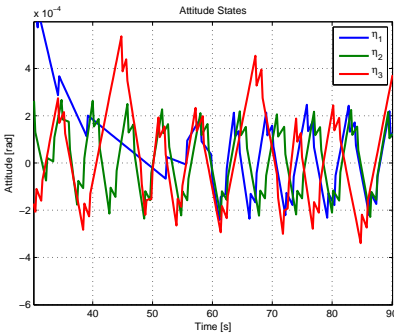
(a) Attitude response
