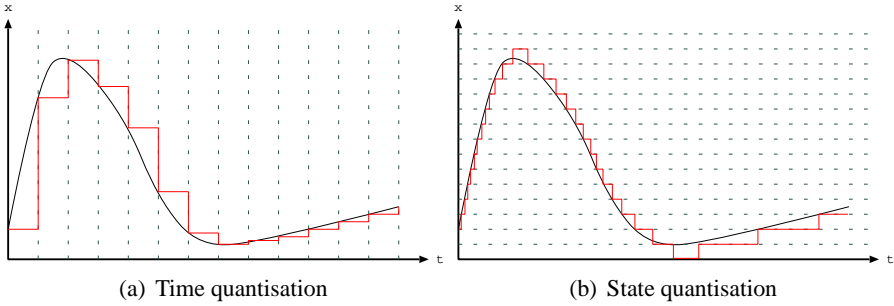
Figure 3.1: Time and state quantisation. The black line is the continuous state evolution and the red line is the discretised state evolution.
