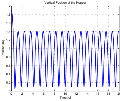
(a) Vertical position
