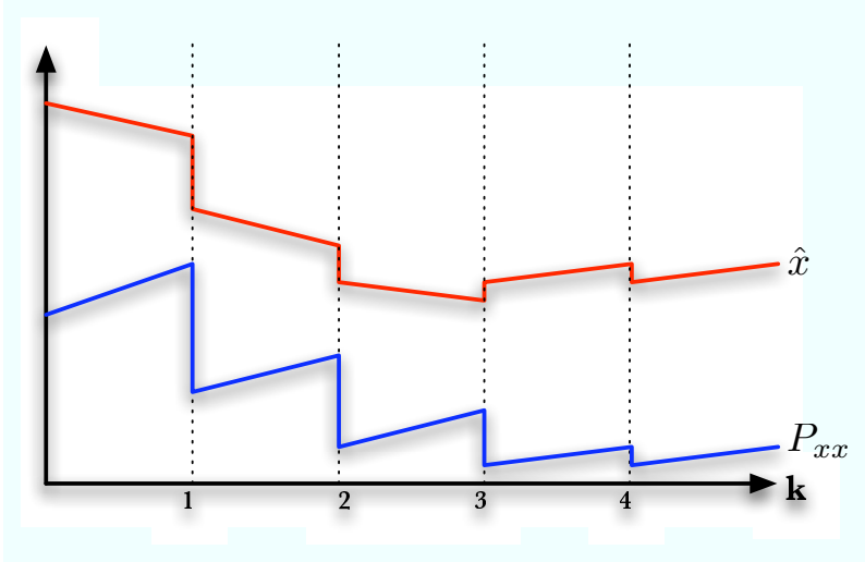
Figure 4.1: Propagation of state (red) and covariance (blue) in the EKF algorithm. New measurement arrive at sample times.
