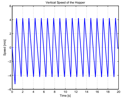
(b) Vertical velocity
