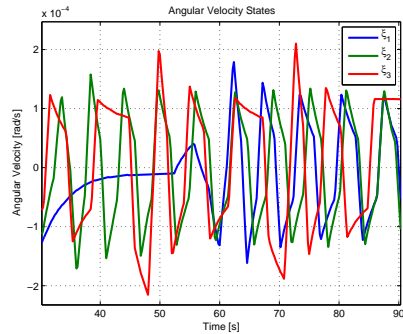
(b) Angular velocities
