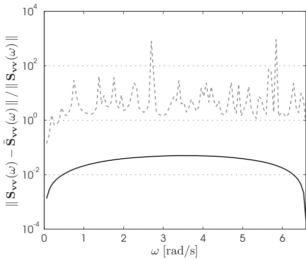
Fig. 5: Relative error of Euclidean norm of modified cross-spectral density matrix. —: \tilde{S}_{\mathbf{v}\mathbf{v}}(\omega) given by Eq. (20). - - : \hat{S}_{\mathbf{v}\mathbf{v}}(\omega) given by Eq. (15).
