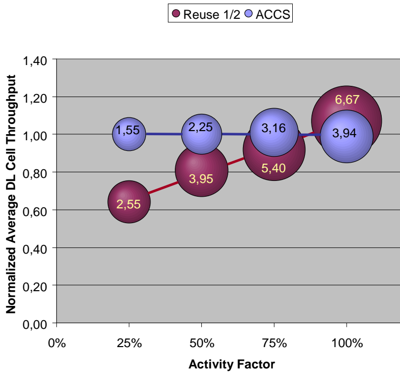
Figure 5 Simulation results for the 100 MHz configuration for variable deployment density levels.
