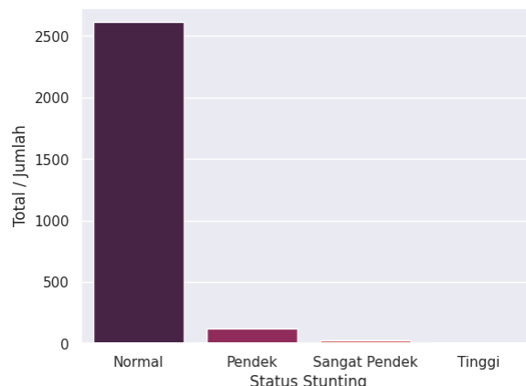
Gambar 3 Data Imbalance
