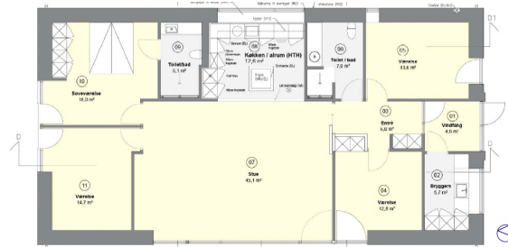
Figure 2. Floor plan
