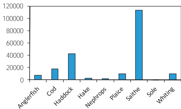
2007 catches (tonnes) of the main species by all otter trawls >100mm mesh for the North Sea, eastern Channel and Skagerrak (ICES areas IIIA, IV and VIId) (Source: STECF)
