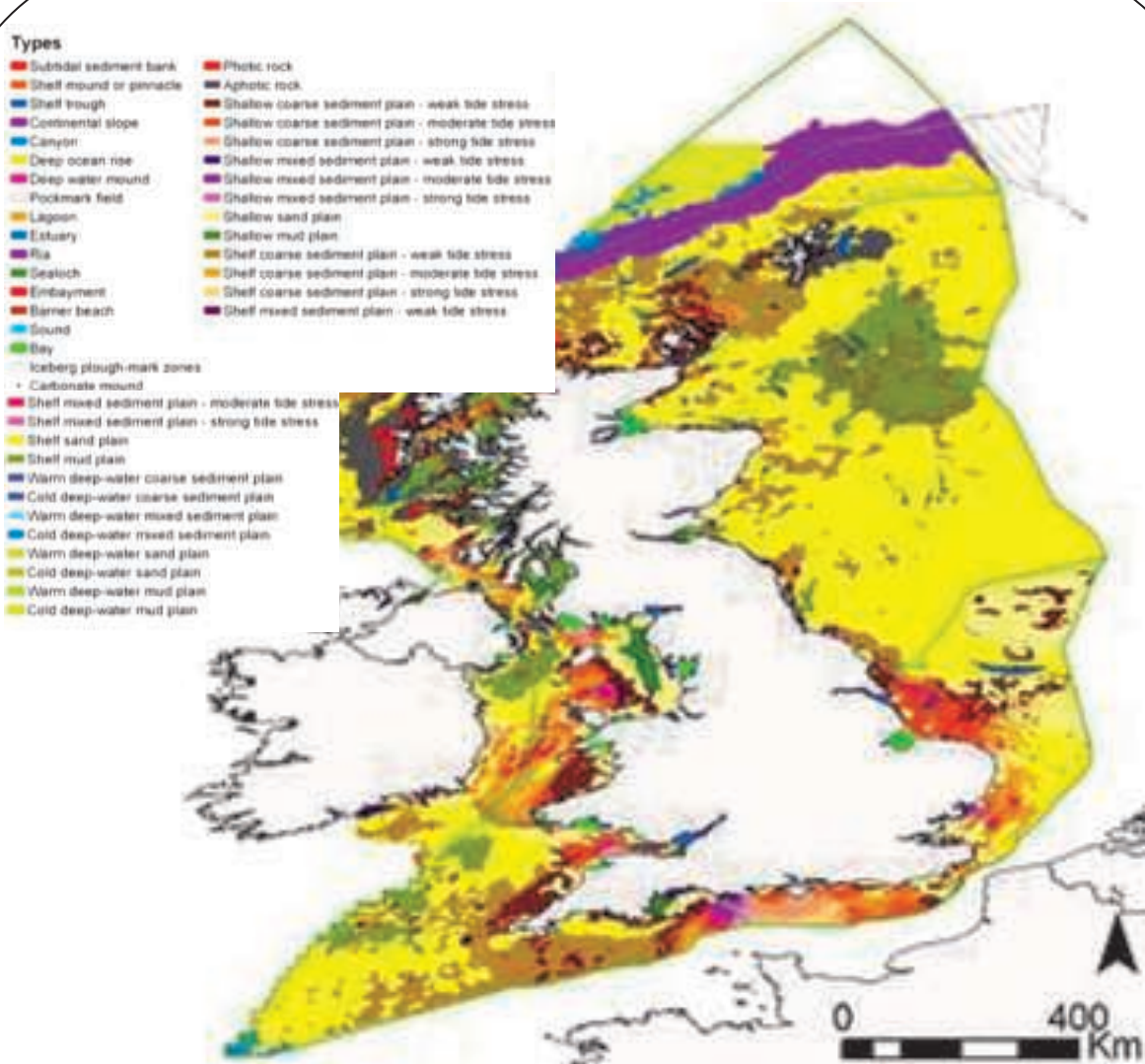
The distribution of marine landscapes around the UK derived from the combination of sediment and bathymetry maps with information on tidal stress and a limited amount of ground truthing.
