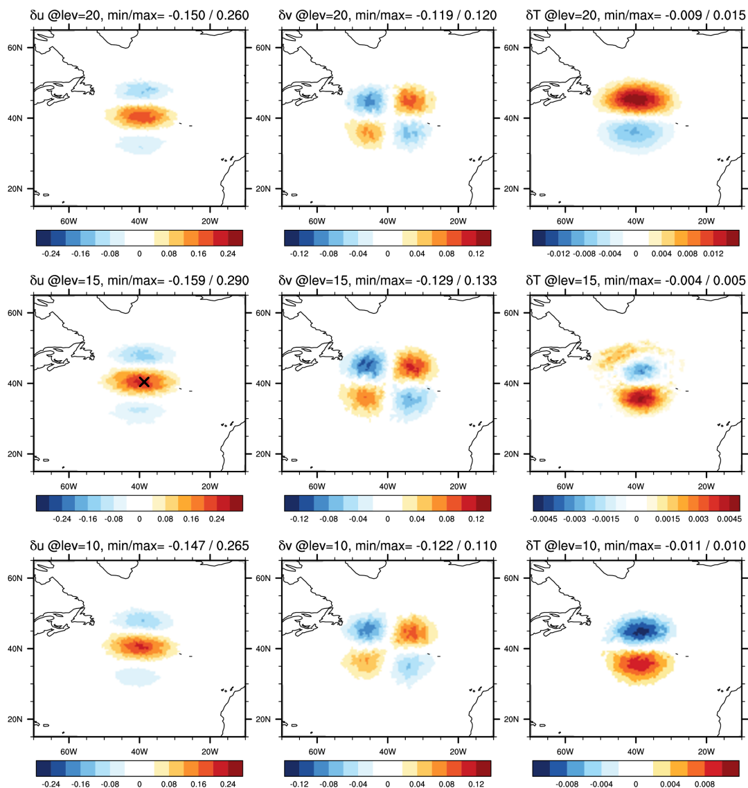
Figure 8. Same as Fig. 7, except from a single zonal wind observation with 1 \text{ ms}^{-1} innovation and 1 \text{ ms}^{-1} observation-error standard deviation.
