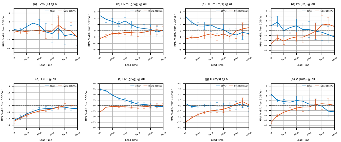
Figure 13. Relative RMSE changes as a function of forecast lead time for (upper row) near-surface and (lower row) three-dimensional variables, compared to 3DEnVar experiment. Shown are (a) T at 2 m, (b) q at 2 m, (c) zonal wind at 10 m, (d) p_s , (e) T , (f) q , (g) zonal, and (h) meridional winds. Statistics are aggregated over 27 extended forecasts with 95 % confidence intervals.
