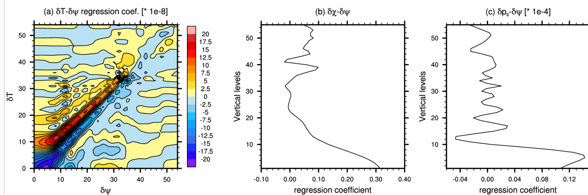
Figure 1. Regression coefficients near 34.8^\circ N between (a) \delta T and \delta\psi [ K(m^2s^{-1})^{-1} ], (b) \delta\chi and \delta\psi [ (m^2s^{-1})(m^2s^{-1})^{-1} ], and (c) \delta p_s and \delta\psi [ Pa(m^2s^{-1})^{-1} ]. These are the nonzero elements at this mesh cell of the submatrices L , M and N , respectively, of K 2 [see Eq. (4)].
