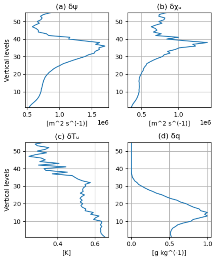
Figure 3. Horizontally averaged standard deviations for (a) \delta\psi , (b) \delta\chi_u , (c) \delta T_u , and (d) \delta q . The horizontally averaged standard deviation for \delta p_{s,u} is 53.05 Pa.
