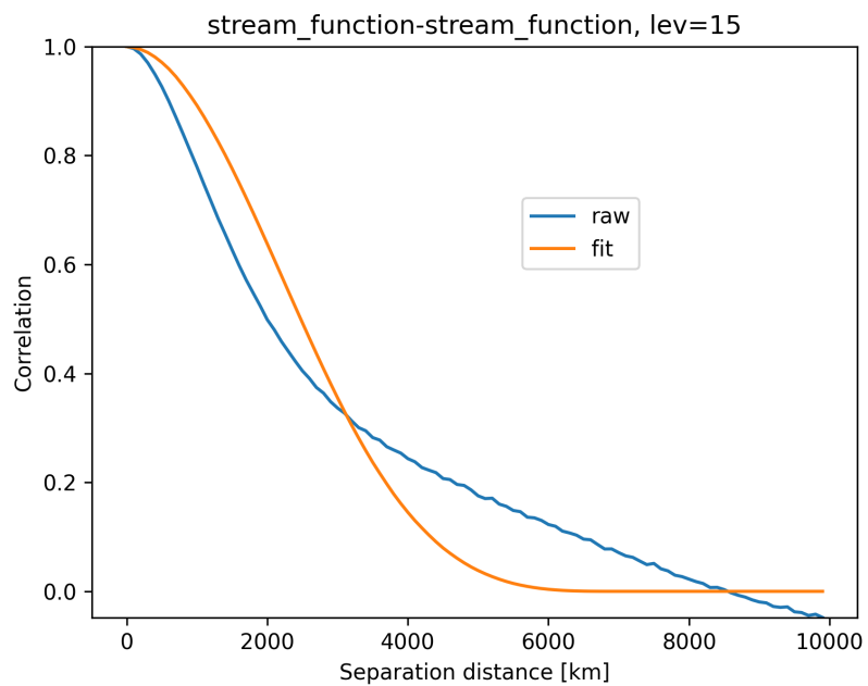
Figure 6. The isotropic correlation function for \delta\psi on the 15th model level, based on the sample of forecast differences (blue). Also shown is the correlation function assumed in BUMP (orange) using the length scale the gives the best fit to the sample-derived correlation.
