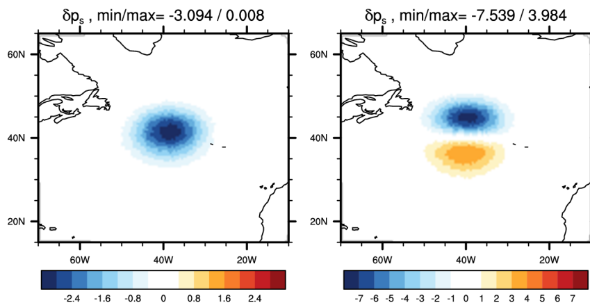
Figure 9. Analysis increments for p_s (left) from a single temperature observation with 1 K innovation and 1 K observation-error standard deviation and (right) from a single zonal wind observation with 1 \text{ms}^{-1} innovation and 1 \text{ms}^{-1} observation-error standard deviation
