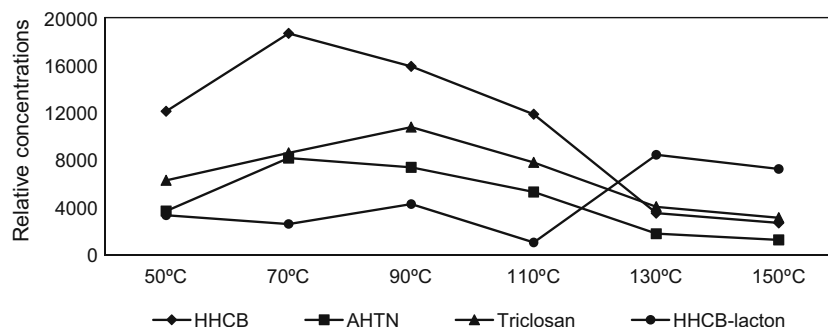
Fig. 2 Relative concentrations of HHCB, AHTN, HHCB–lactone and triclosan obtained by ASE extractions of sludge homogenates at different temperatures
