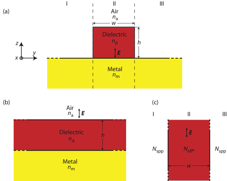
Figure 2.1: (a) Cross-sectional view of the DLSPPW structure. (b) The three-layer slab waveguide structure considered in the first step of the EIM, with finite height h of the dielectric layer. (c) The three-layer structure considered in the second step of the EIM, where the effective index found in the first step represents the middle layer of width w . The coordinate system used is also shown along with the orientation of the main component of the electric field in the case of TM (SPP) modes.
