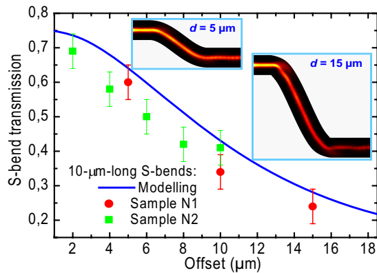
Fig. 2. S-bend transmission dependence on the offset distance between the arms for the 10- \mu\text{m} -long S-bends ( \lambda = 1,550\text{ nm} ) determined experimentally from SNOM images (similar to those shown in Fig. 1) and by modeling with 3D-FEM simulations. Insets show calculated intensity distributions in two S-bends with different offsets that should be compared to the optical images shown in Fig. 1(e) and Fig. 1(i). The error bars are obtained from single measurements and, thus, represent the uncertainty in each measurement due to variations in the optical signal.
