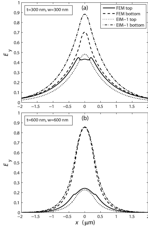
FIG. 13. Lateral profiles of the vertical component of the electric field calculated by utilizing the EIM-1 and the FEM. The bottom profiles are taken 50 nm from the gold-polymer interface and the top profiles are taken 50 nm from the top of the ridge. The field profiles are shown for a t=300 nm, w=300 nm and for a t=600 nm, w=600 nm ridge SPP waveguide.
