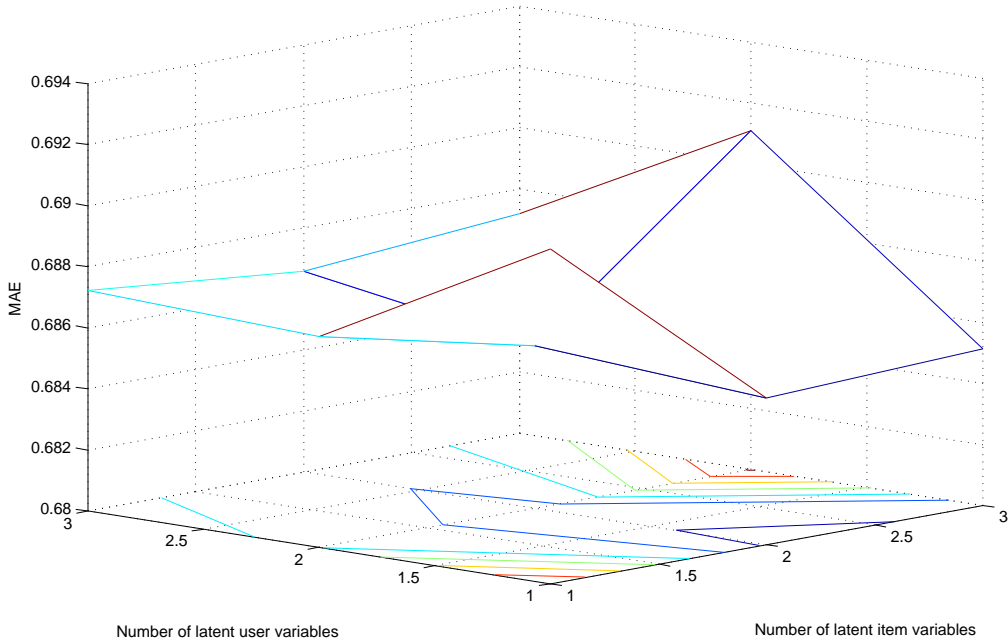
Figure 4: The figure shows the MAE as a function of the number of latent variables. A minimum (0.685) is found at |\mathbf{U}| = 1 and |\mathbf{M}| = 2 .
