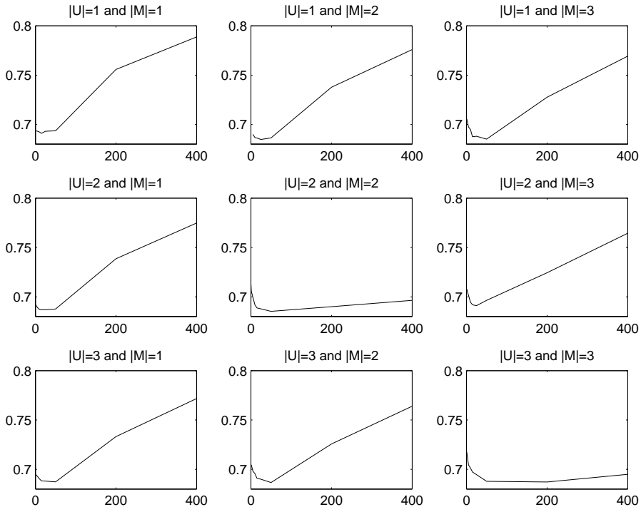
Figure 3: The figure shows the MAE as a function of the prior precision for the regression vectors. Each plot corresponds to a certain configuration of the number of latent variables.
