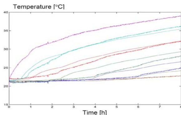
Figure 5 Test A. Continuous heating.
