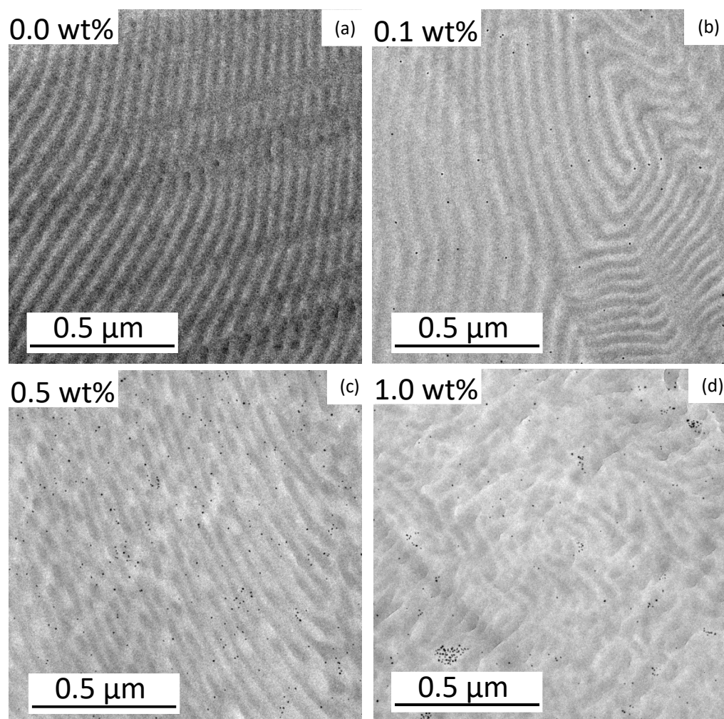
Figure 2. TEM images of the BCP films with FePt-NPs compositions of 0 wt% (a), 0.1 wt% (b), 0.5 wt%, (c), and 1.0 wt% (d). Within the morphology, the PS domains appear electron opaque (dark) and the PMMA domains are light. The NPs are represented by dark dots.
