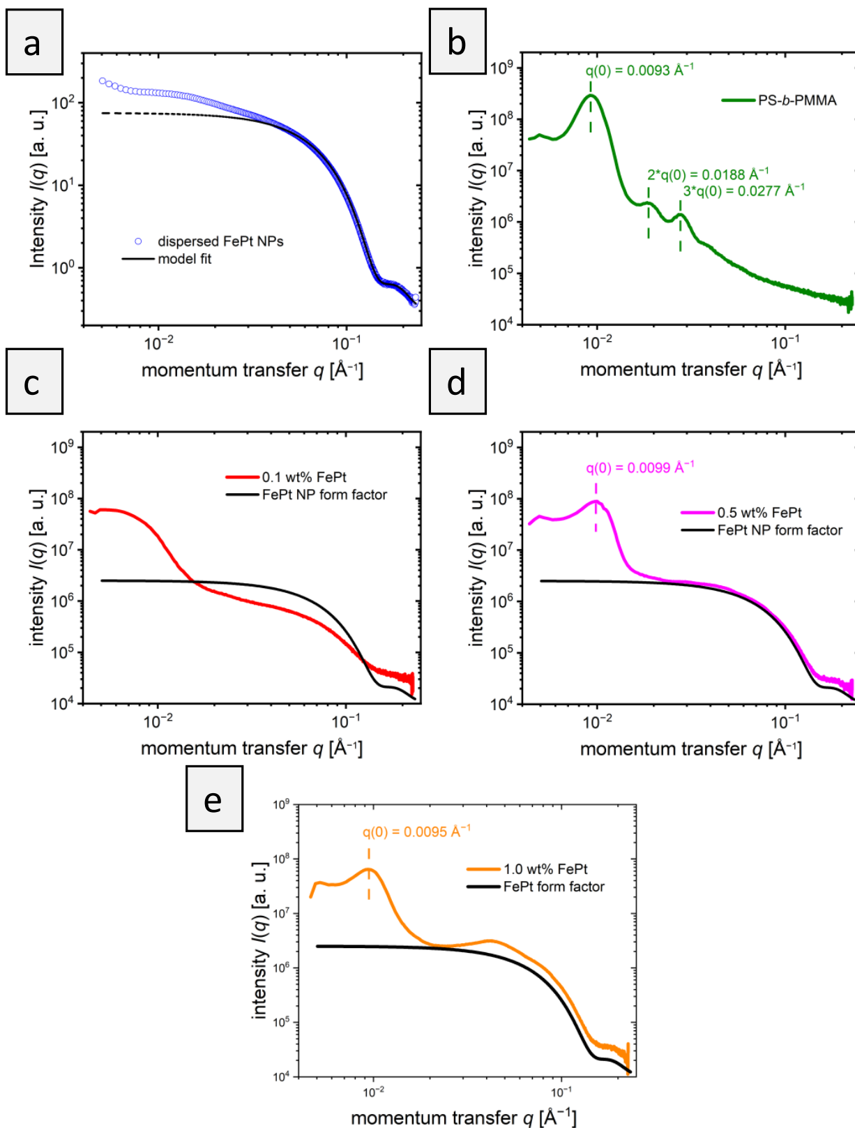
Figure 4. SAXS curves of the PS- b -PMMA films with FePt particles. (a) FePt dispersed in toluene. The solid line shows a fit according to Equation (1), the dotted line is an extrapolation to low q -values. (b) PS- b -PMMA film in the absence of NPs. (c) 0.1 wt% FePt-NPs in PS- b -PMMA, (d) 0.5 wt% FePt NPs in PS- b -PMMA, and (e) 1.0 wt% FePt NPs in PS- b -PMMA. In (c–e), the solid black lines denote the form factor of the FePt NPs.
