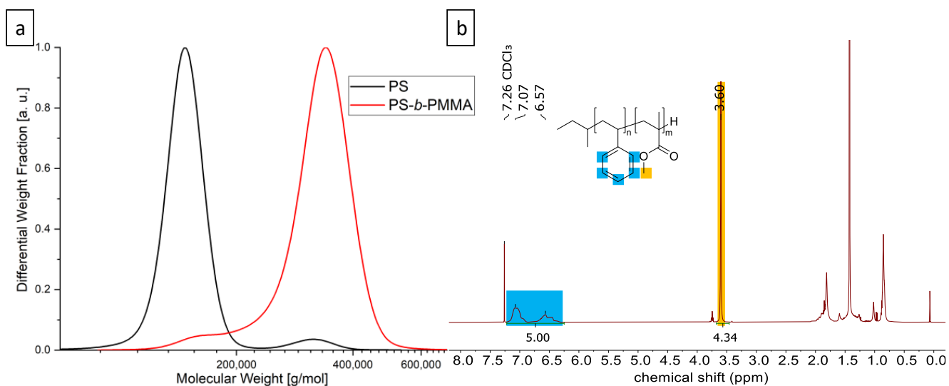
Figure 1. Analytical data of the UHMW PS- b -PMMA block copolymer. (a) SEC was measured in THF vs. PS standards; (b) 1 H-NMR was measured in CDCl 3 and referenced to the solvent peak.
