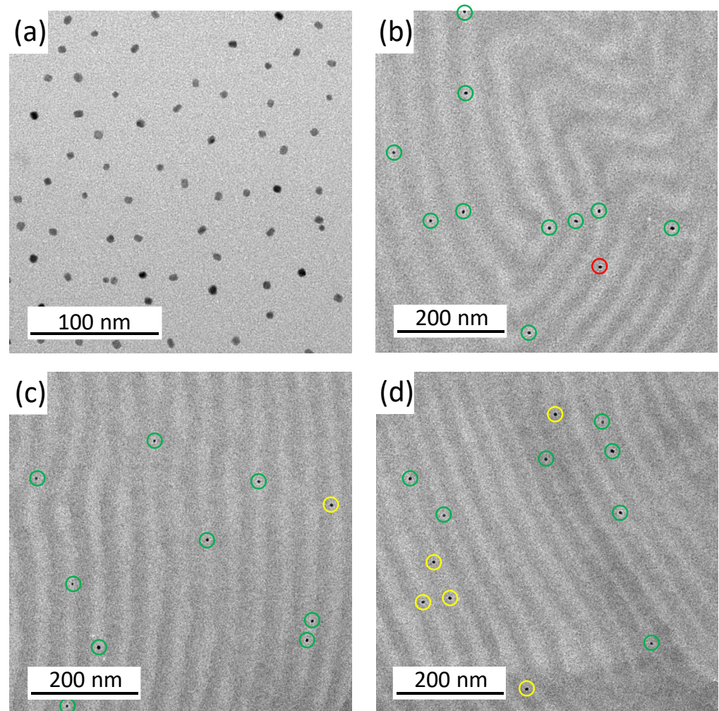
Figure 3. TEM images of the BCP films with 0.1 wt% FePt NP. Figure (a) shows the pure FePt NPs, while Figure (b–d) are different images of the lamellar PS- b -PMMA morphology with 0.1 wt% FePt NPs. The particles are marked with a green ring in the light PMMA phase, red in the dark PS phase, and yellow on the boundary.
