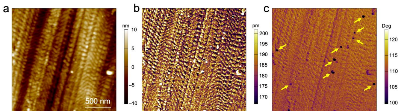
Figure 5. Bimodal magnetic force microscopy of the block copolymer structure with embedded FePt nanoparticles (highlighted with yellow arrows). (a) Topography image, (b) amplitude, and (c) phase shift of the second eigenmode.
