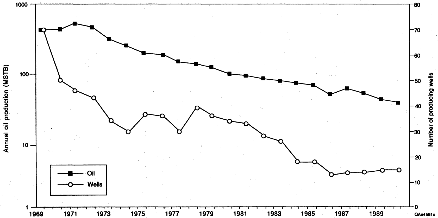
Figure 28. Trends in annual oil production and number of producing wells in Rincon field from 1968 to 1990.
