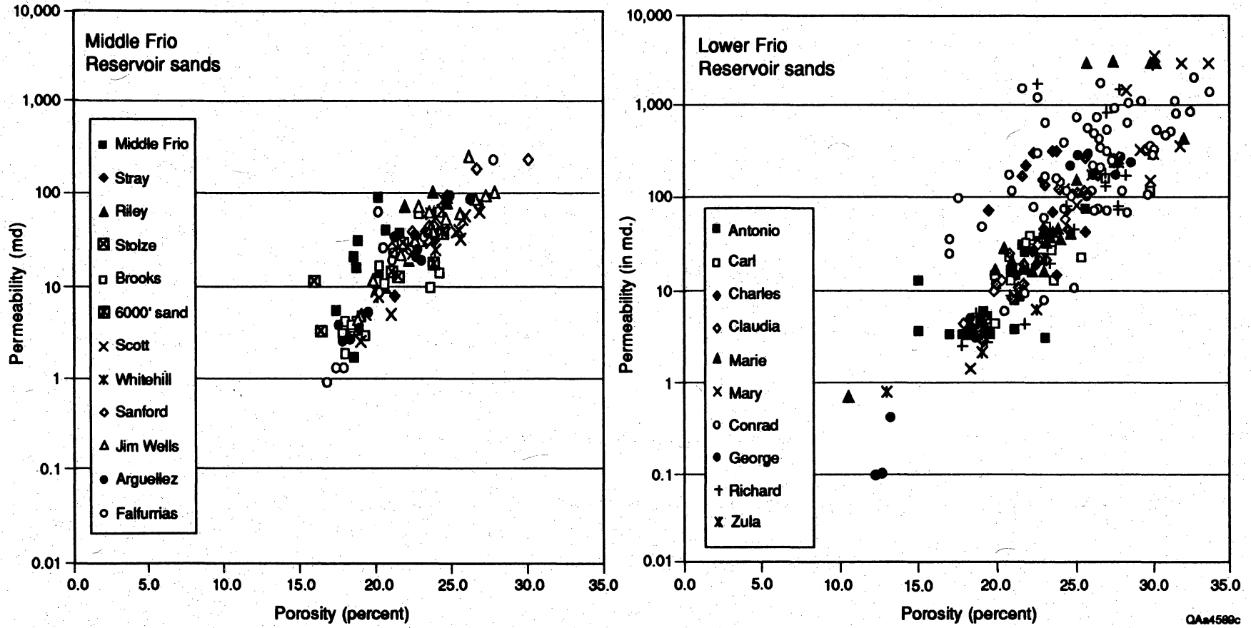
Figure 44. Representative reservoir variability illustrated on a porosity/permeability cross plot for middle and lower Frio zones in T-C-B field.
