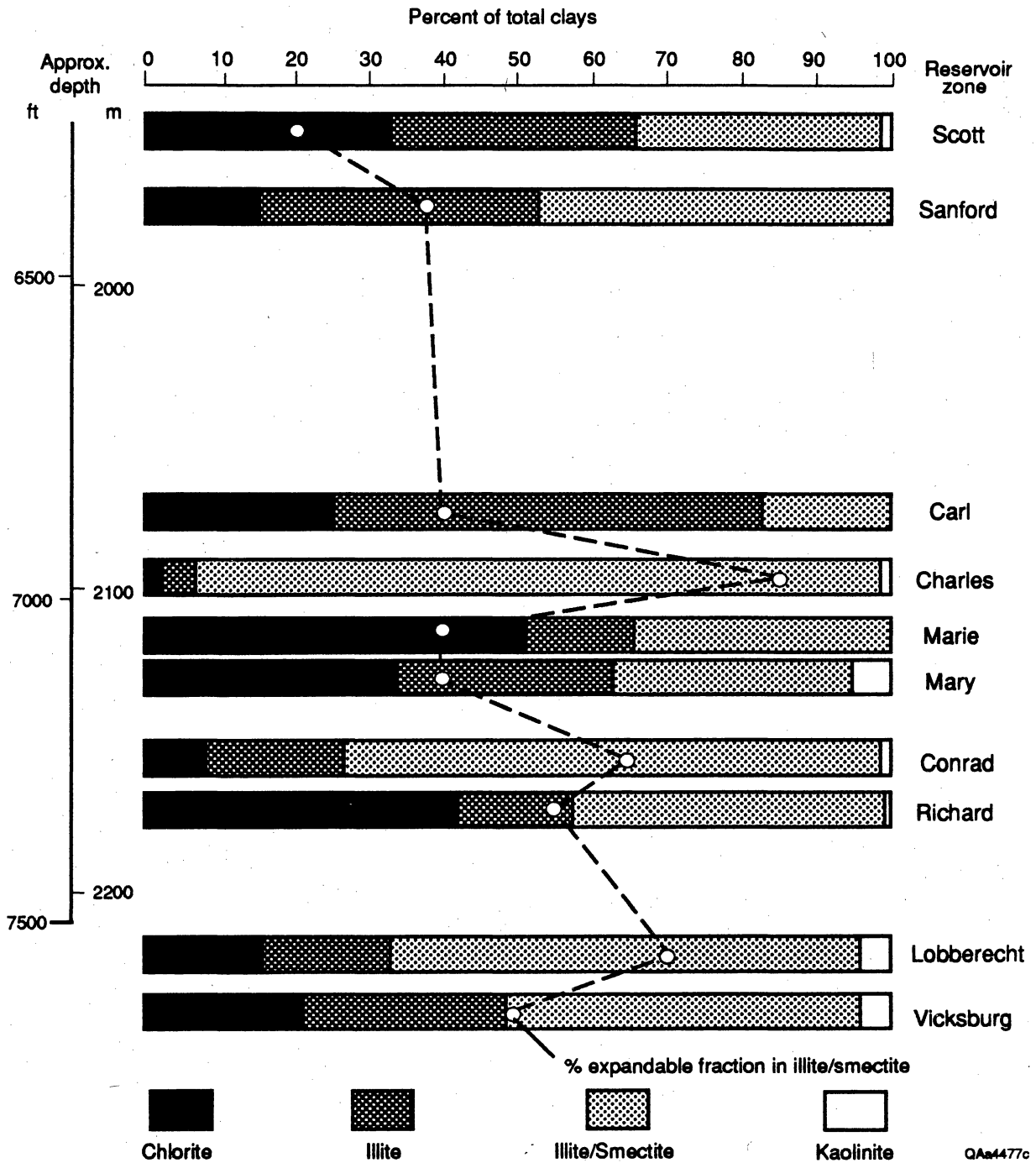
Figure 45. Bar graph illustrating clay mineralogy within the less than 2\ \mu -size fraction of sidewall core samples from various T-C-B reservoirs. Relative abundances of chlorite, illite, mixed-layered illite-smectite, and kaolinite are plotted, as is the percent of expandable clay in the mixed-layered illite-smectite fraction. The dominance of chlorite and moderately expandable illite-smectite results in reservoirs that are susceptible to damage from drilling and acidizing fluids.
