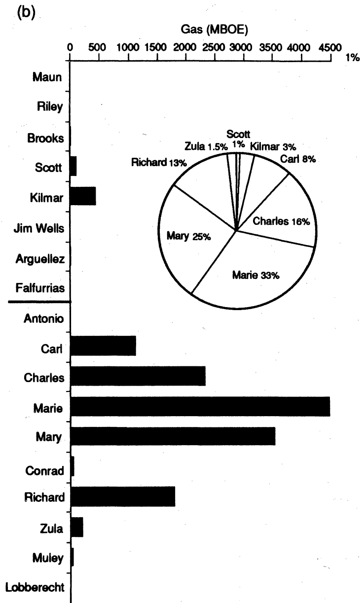
Figure 40. Summary of cumulative (A) oil and (B) gas production from Mobil leases from 1967 to 1992, illustrating the relative importance and stratigraphic position of Frio Formation reservoir intervals. The Marie and Mary sands are equivalent to the prolific 21-B interval, which has produced more than 20 million barrels (MMbbl) of oil throughout the life of the T-C-B field.
