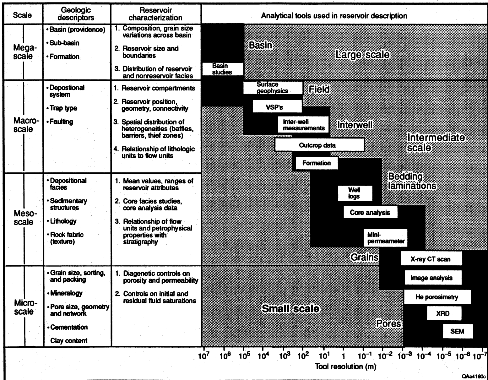
Figure 3. Analytical tools used in the description of reservoir heterogeneity at various scales. Data from Worthington (1991) and Jackson and others (1993).
