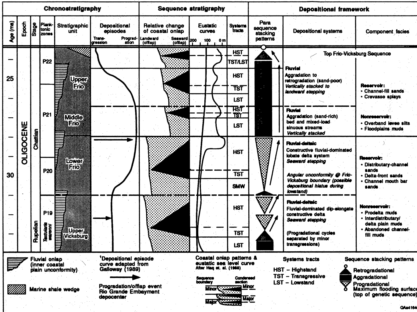
Figure 12. Chronostratigraphic, sequence-stratigraphic, and sediment stacking pattern relationships of the upper Vicksburg–Frio genetic stratigraphic interval in the lower Gulf Coast of South Texas. The relative degree of sediment progradation versus marine transgression illustrated on the depositional episode curve constructed by Galloway (1989) is compared with the relative coastal onlap and offlap patterns and eustatic sea-level curve for the Middle and Late Oligocene (from Haq and others, 1988). Comparison of the period of maximum progradation of the Vicksburg–Frio delta sequence identified on the depositional episode curve with the major sea-level drop in the middle Oligocene suggests an offset of at least a few million years and is interpreted to reflect a significant tectonic imprint on sedimentation (Galloway, 1989). Stratigraphic data from Galloway (1977), Galloway and others (1982), Coleman and Galloway (1990), and Xue and Galloway (1991).
