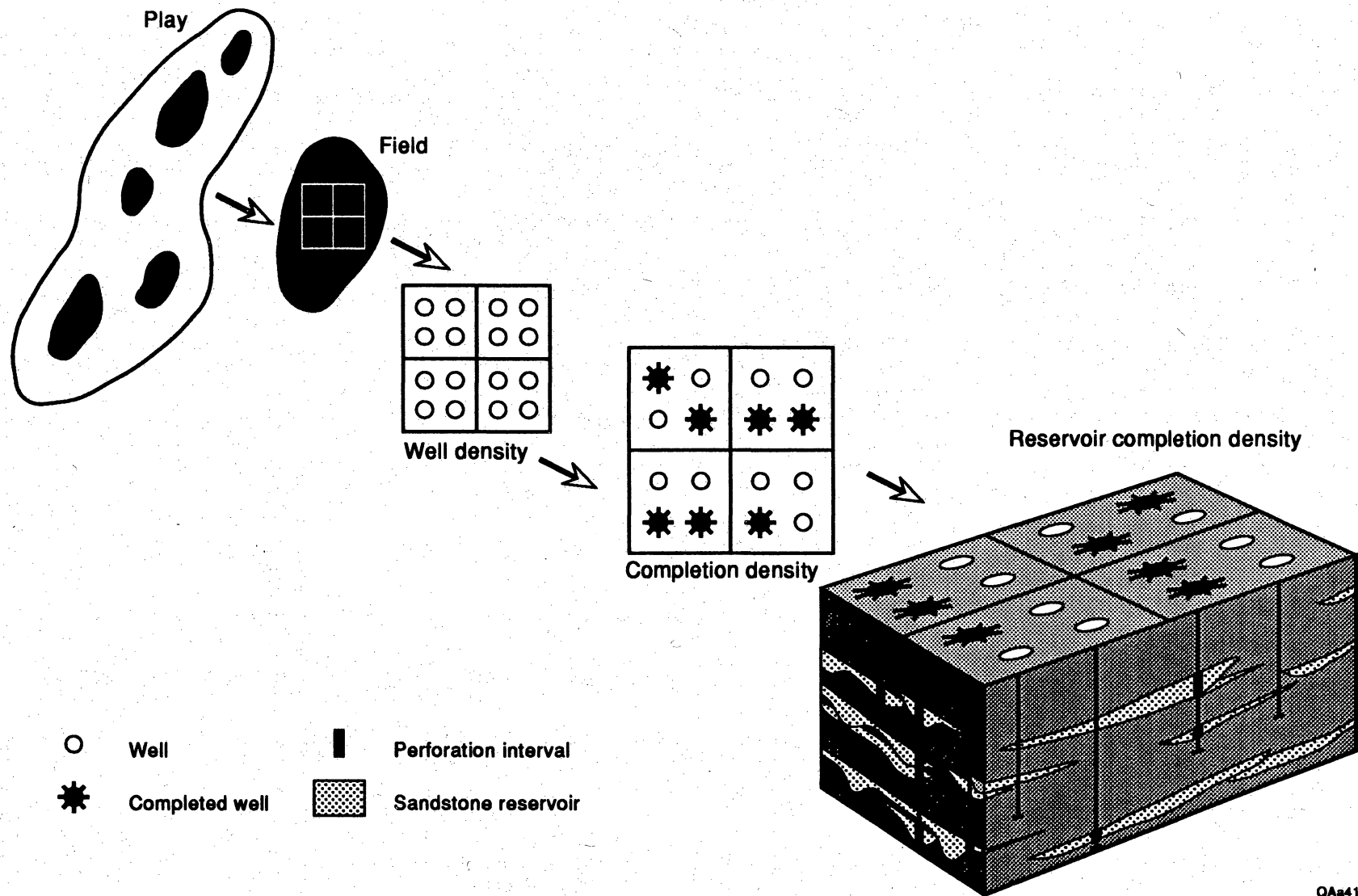
Figure 5. Illustration of various field and reservoir production parameters that can be used in the evaluation of reservoir infill potential within a play, field, or reservoir. Density of completions is identified within a field area and subsequently for individual reservoir zones. The distribution of completions per reservoir is used to identify which zones have lower completion densities and therefore higher potential for incremental recovery of additional reserves. In the example shown here, reservoir B has a lower completion density than that of zones A and C and may possess greater potential for containing untapped or partially drained reserves.
