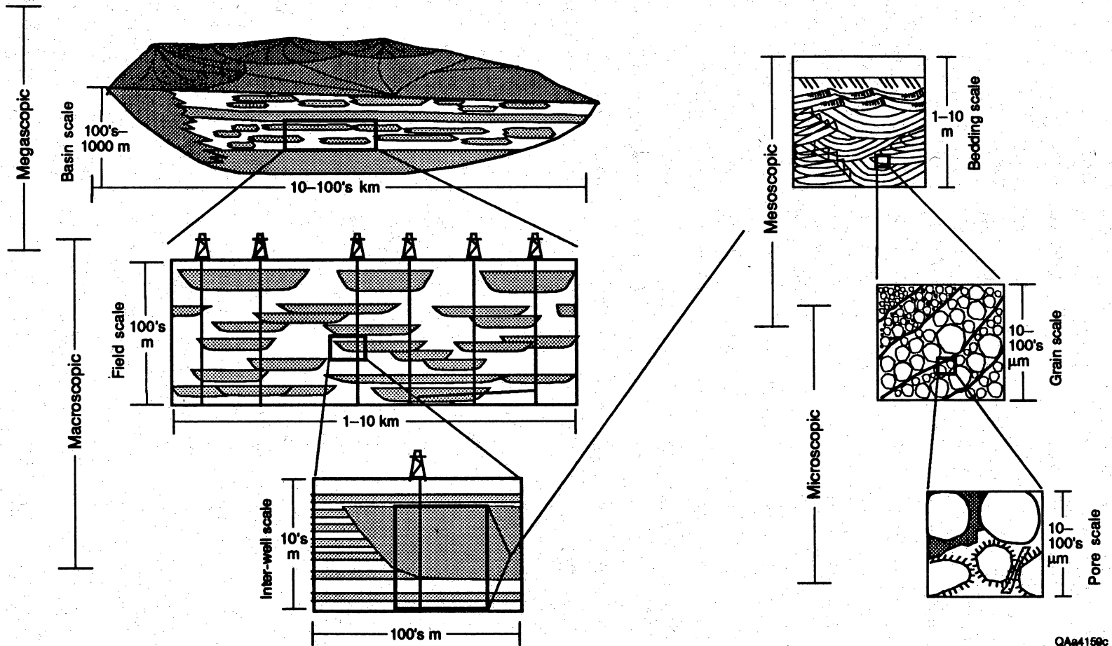
Figure 2. Examples of scales associated with the various levels of heterogeneity present in fluvial-deltaic reservoirs. Compiled from Weber (1986) and Miall (1988).
