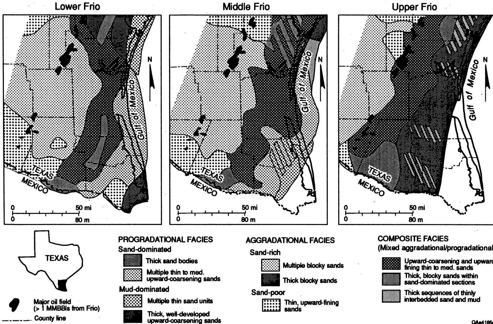
Figure 11. Distribution of aggradational and progradational sequences of the Frio Formation along the Vicksburg Fault Zone oil play (map distribution from Galloway and others, 1982). The Frio sediments near the Vicksburg Fault Zone were deposited primarily in moderate- to high-sinuosity mixed-load stream environments of the Gueydan fluvial system. Based on log facies maps by Galloway and others (1982).
