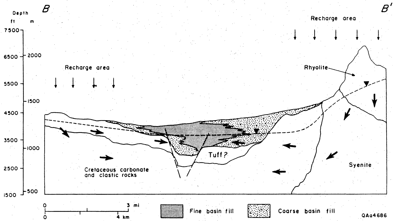
Figure 37. Conceptual hydrogeologic cross section B-B'.
