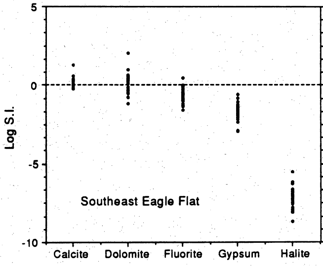
Figure 12. Range of saturation indices of calcite, dolomite, fluorite, gypsum, and halite for northwest Eagle Flat, Red Light Draw, and southeast Eagle Flat.
