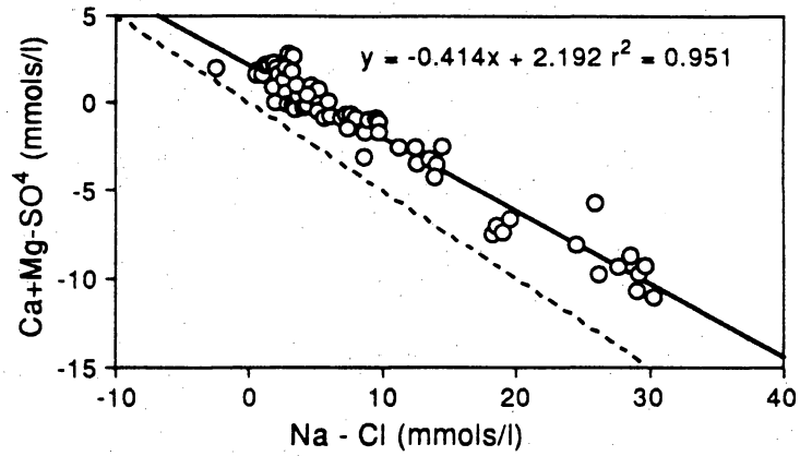
Figure 20. Binary plot of (Ca + Mg - SO_4) versus (Na - Cl) . The quantity (Ca + Mg - SO_4) represents the molar concentration of Ca and Mg not associated with sulfates. The points for a downward trend interpreted to be the result of the loss of Ca and Mg in exchange reactions for Na. The quantity (Na - Cl) represents excess Na, as described in the text and in figure 14.
