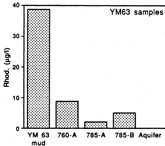
Figure 33. Comparison of conservative anions and rhodamine dye in drilling mud, recovery waters from well test intervals, and water collected from the completed well at YM-63. Two test samples collected at 785 ft (785-a and 785-b) and one test sample collected at 760 ft (760-a). Results of analysis of a drilling mud sample (YM-63 mud) and a sample from the completed well are shown. Comparisons between conservative anions and rhodamine dye indicate that almost 3/4 of recovery water is formation water at 760 and 785 ft. These results, along with recovery rates indicate considerable storage and yield from the semiconfining unit, or semiconfining interbeds at YM-63. These results imply conditions similar to conceptual models 2 or 3 (fig. 31) at YM-63.
