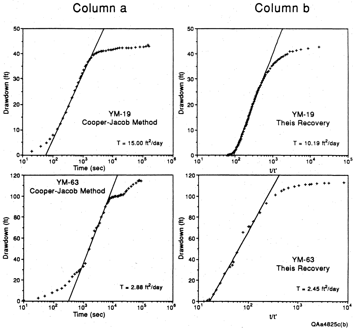
Figure 10 (continued). Semilog match of straight line segments of drawdown and recovery data for wells in northwest Eagle Flat. Semilog analysis of time-drawdown data provided by the Cooper-Jacob (1946) method (column a). Semilog analysis of recovery data provided by the Theis (1935) recovery method (column b). For Cooper-Jacob (1946) interpretations, wellbore storage effects during early time drawdowns probably cause the nonlinear curve segment to drift to the left of the linear segment. The sharp inflection away from the linear segment during late time drawdowns is due to vertical leakage from the semipervious confining layers. The straight line segment matched during intermediate times represents the withdrawal of water from storage from the confined aquifer, no part of which was contributed from the semipervious confining layers (i.e., during intermediate times, all the water pumped comes from storage in the confined aquifer). After intermediate times, leakage from the semipervious units forms a significant part of the water pumped.
