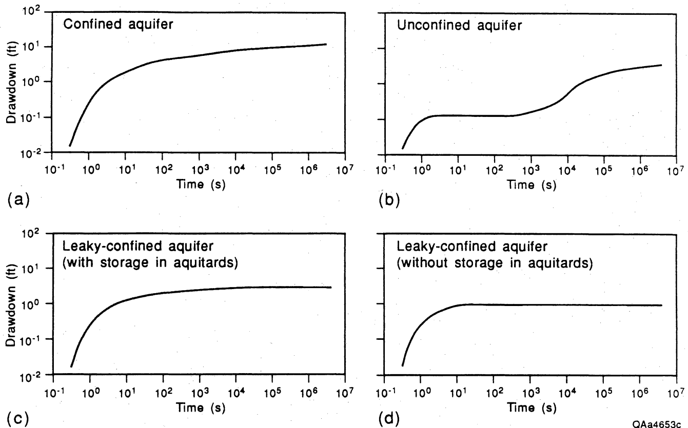
Figure 4. Representative time-drawdown curves for confined, leaky confined, and unconfined aquifers observed during aquifer testing. The nonequilibrium time-drawdown curve for a fully confined aquifer is a parabola (a). The time-drawdown curve for an unconfined aquifer often is an s-shaped curve (b). The time-drawdown curves for leaky confined aquifers (c and d) are suppressed parabolas because a leaky confined aquifer is replenished by vertical flow from lower permeability bounding strata.
