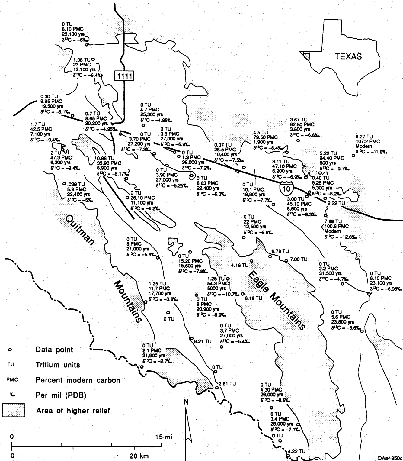
Figure 22. Map of 3 H, 14 C and δ 13 C in southern Hudspeth County ground water. Carbon-14 is shown as percent modern carbon (PMC), along with uncorrected ages. Tritium is reported as tritium units. δ 13 C is measured with respect to PDB standard.
