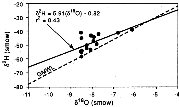
Figure 27. Plot of \delta^2\text{H} versus \delta^{18}\text{O} for low-TDS samples in Red Light Draw.
