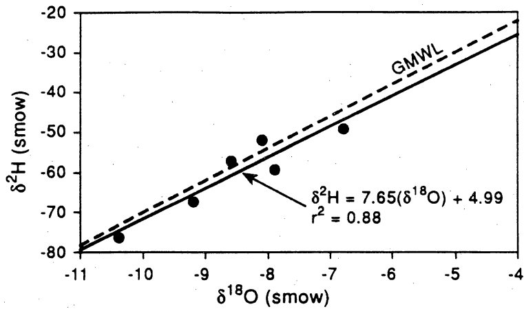
Figure 26. Plot of \delta^2\text{H} versus \delta^{18}\text{O} for locations within the high-TDS zone in lower Red Light Draw.
