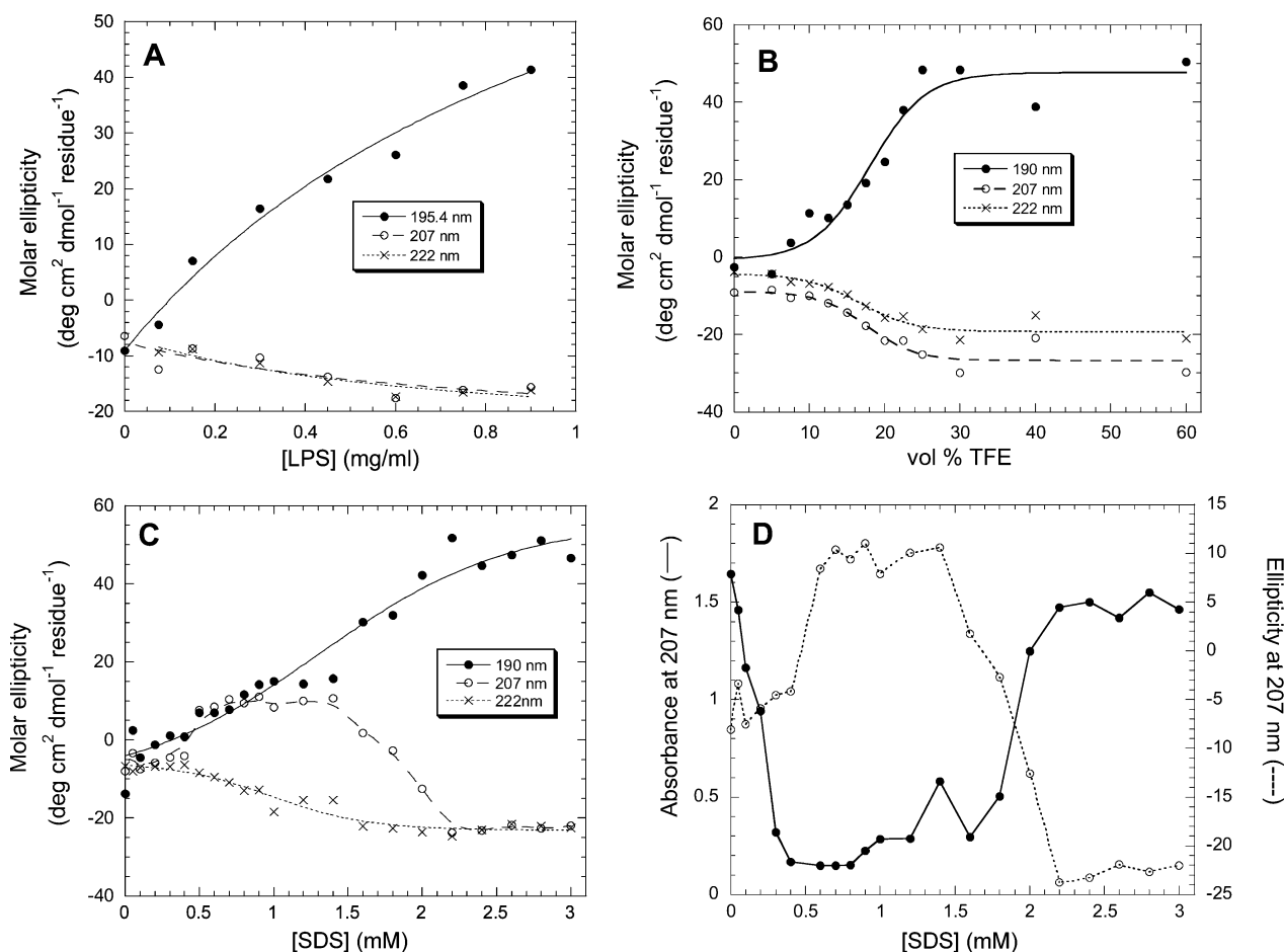
FIGURE 2: (A) Molar ellipticity of 40 μM Novispirin as a function of lipopolysaccharide from E. coli . Data fitted to eq 1 (results in Table 3). (B) Molar ellipticity of 40 μM Novispirin as a function of TFE. Data fitted to eq 2. (C) Molar ellipticity of 40 μM Novispirin as a function of SDS. Data for 190 and 222 nm are fitted to eq 2, while data at 207 nm are joined up for clarity. Data are restricted to 0–3 mM for clarity; there are no further transitions beyond 3 mM SDS. Increasing the Novispirin concentration to 400 and 1140 μM leads qualitatively to the same transitions, although the spectral changes occur later at higher SDS concentrations. (D) Solubility of 40 μM Novispirin as a function of SDS concentration. Novispirin was incubated at different SDS concentrations and centrifuged, and the absorbance (joined lines) and ellipticity at 207 nm (stippled lines) of the supernatant were measured.
