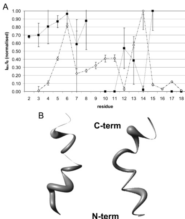
FIGURE 7: (A) Influence of paramagnetic Mn^{2+} ions on relative signal intensity of Novispirin in SDS at 50 °C (closed squares) and LTAB at 25 °C (open diamonds). The top graph shows I_{Mn}/I_0 plotted vs the peptide sequence, where I_{Mn} is the signal intensity in a clean-TOCSY spectrum (41) of 20 ms mixing time with a 15 kHz spin-lock and a WATERGATE water suppression (40) after addition of 0.5 mM Mn^{2+} , and I_0 is the signal intensity before addition of Mn^{2+} . The highest ratio occurring in each of the samples was normalized to 1, since no comparisons of absolute signal intensity between two different samples could be made. In general, signal intensity ratios are far weaker for LTAB than for SDS. (B) Visualization of the data using the structures for Novispirin in SDS (left) and LTAC (right). The backbone is represented by a spline function, whose radius is proportional to the I_{Mn}/I_0 value plotted in the top graph. The thinner the curve, the more this individual residue is influenced by Mn^{2+} ions.
