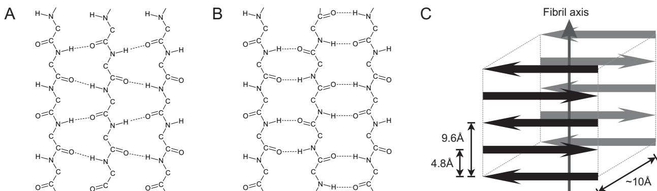
Figure 5. Parallel (A) and anti-parallel (B) pleated sheets [96]. The cross- \beta structure consist of laminated pleated sheets (shown as anti-parallel) running along the fibril direction with strands oriented perpendicular to the fibril axis. Adapted from [97].
