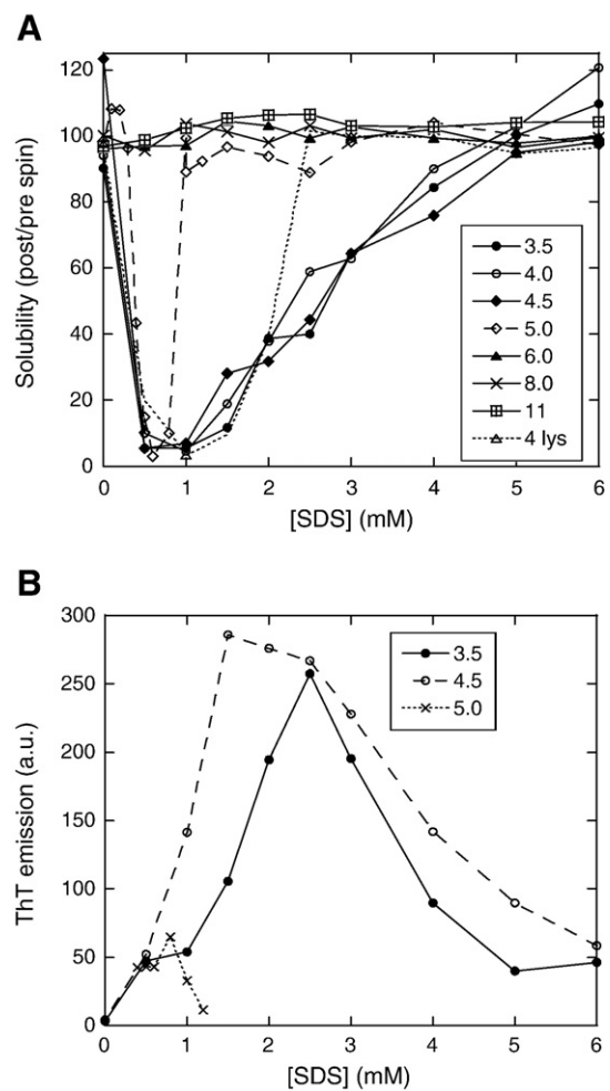
Fig. 5. (A) Solubility of 20 \mu\text{M} S6 as a function of SDS at pH 3–11. Solubility measured as the ratio of the Trp emission intensity of the supernatant (excitation 280 nm, emission 350 nm) before and after centrifugation. Solubility of lysozyme (lys) at pH 4 also shown. (B) ThT fluorescence of pellets obtained from panel A (excitation 350 nm, emission 485 nm) by centrifugation and resuspension in the same volume and same buffer as in (A) but without SDS.
