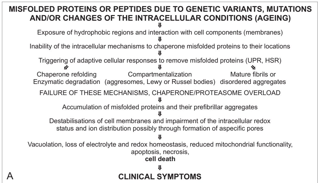
Figure 17. The progression from protein misfolding to clinical symptoms (A [331]) proceeds through several steps. Although the details of the causes of protein misfolding are not known, they likely involve an interplay of numerous factors (B [5]).
