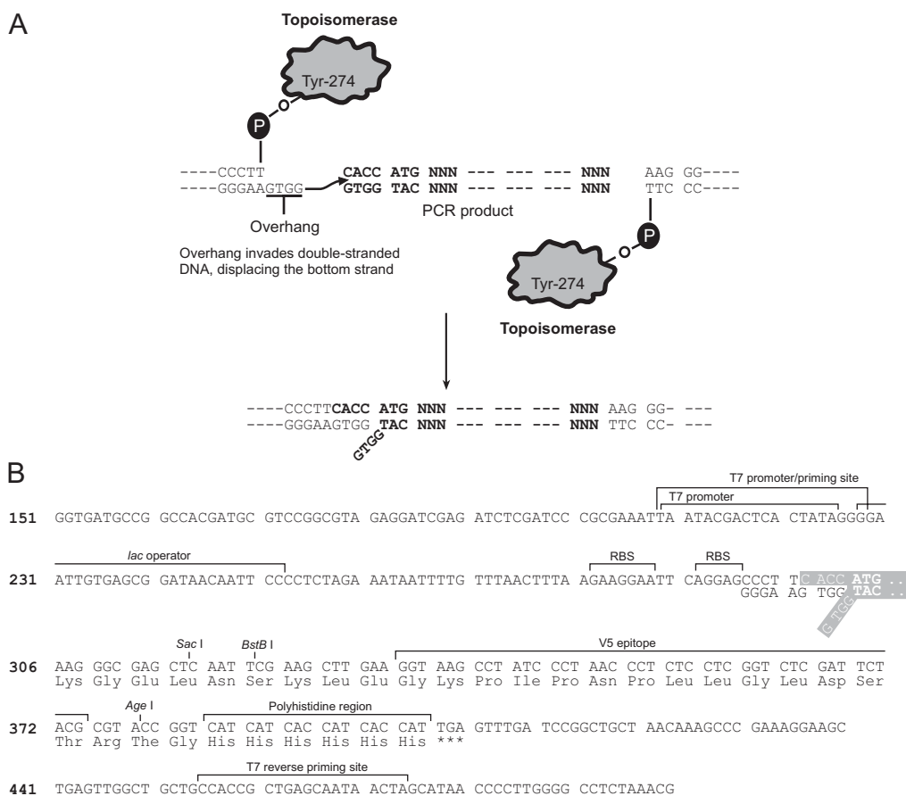
Figure 50. Principle of TOPO cloning (A) and sequence of the cloning region (B) (tools.invitrogen.com/content/sfs/manuals/pettopto_man.pdf).
