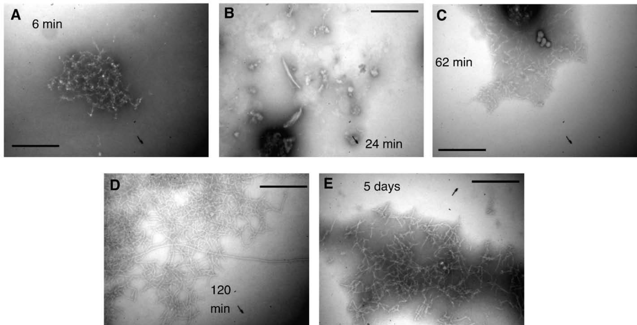
Fig. 3. Time-resolved electron micrographs of 50 \mu\text{M} SerADAN at pH 7.5. Black bar corresponds to 400 \mu\text{m} . (A) Morphology after 6 min. (B) Amorphous structures observed after 24 min. Structures coexistent with structure of the type shown in A. (C) Sample obtained after 62 min contains filaments and amorphous elements. (D) Long, thin filaments of clear morphology obtained after 2 h and frozen for later imaging. (E) Sample obtained and frozen after 5 days aging. Thin filaments persist as dominating structure.
