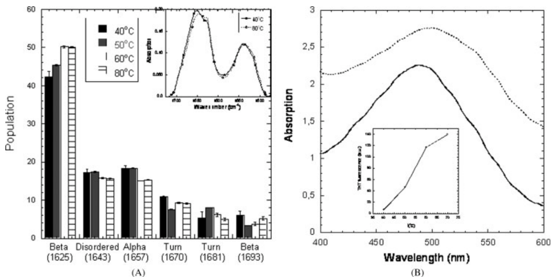
FIGURE 2 A: Secondary structure content of aggregated cutinase at pH 8.0 based on FTIR spectra. Cutinase ( 80 \mu\text{M} ) was incubated at 40–80°C for 15 min. Insert: FTIR spectra of samples incubated at 40 and 80°C. B: Absorption spectra of Congo red alone (joined line) and in the presence of 80 \mu\text{M} cutinase aggregated by exposure to 50°C at pH 8.0 for 15 min (dashed line). Insert: emission intensity of thioflavin T at 485 nm (excitation 450 nm) in the presence of 80 \mu\text{M} cutinase incubated at different temperatures for 15 min at pH 8.0.
