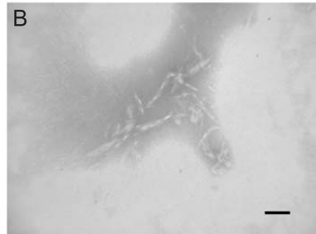
Figure 38. (A) X-ray fibre diffractogram of ThT-positive aggregates of recombinant SerADan, disaggregated in HFIP, incubated at pH 5.5 with shaking. (B) Aggregate morphology by EM. Scale bar corresponds to 90nm. Adapted from [573]
