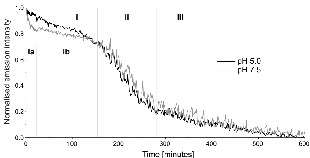
Figure 33. The time-course of SerADan aggregation followed by intrinsic Trp fluorescence falls into three phases. The first phase can be divided further for pH 7.5.
