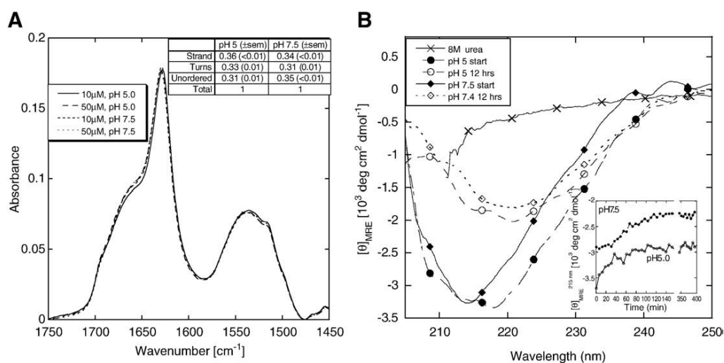
Fig. 4. Secondary structure of aggregated SerADAN. (A) Fourier transform infrared spectroscopy of 10 and 50 \mu\text{M} SerADAN at pH 5.0 and 7.5, aged for 12 h at 10 and 50 \mu\text{M} peptide. The aggregates were washed in water and found to be stable over several days. The secondary structure appears independent of pH and concentration. Table: Estimate of secondary structure content by curve fitting. (B) CD spectra of 50 \mu\text{M} SerADAN in 10 M urea (no buffer) and at pH 5.0 and 7.5 after 50-fold dilution into 0.2 M urea. Immediately after dilution, there is a clear minimum around 215–220 nm, indicative of \beta -sheet structure. The spectra reduce in intensity over the next 12 h but retain minimum around 215–220 nm. Inset: change in molar ellipticity at 215 nm over time when 50 \mu\text{M} SerADAN is diluted into 0.2 M urea from 10 M urea, indicating that most of the ellipticity change occurs over the first 100 min. Ellipticity levels for the two runs have been offset for clarity. Note the lag phase at pH 7.5 which is absent at pH 5.0.
