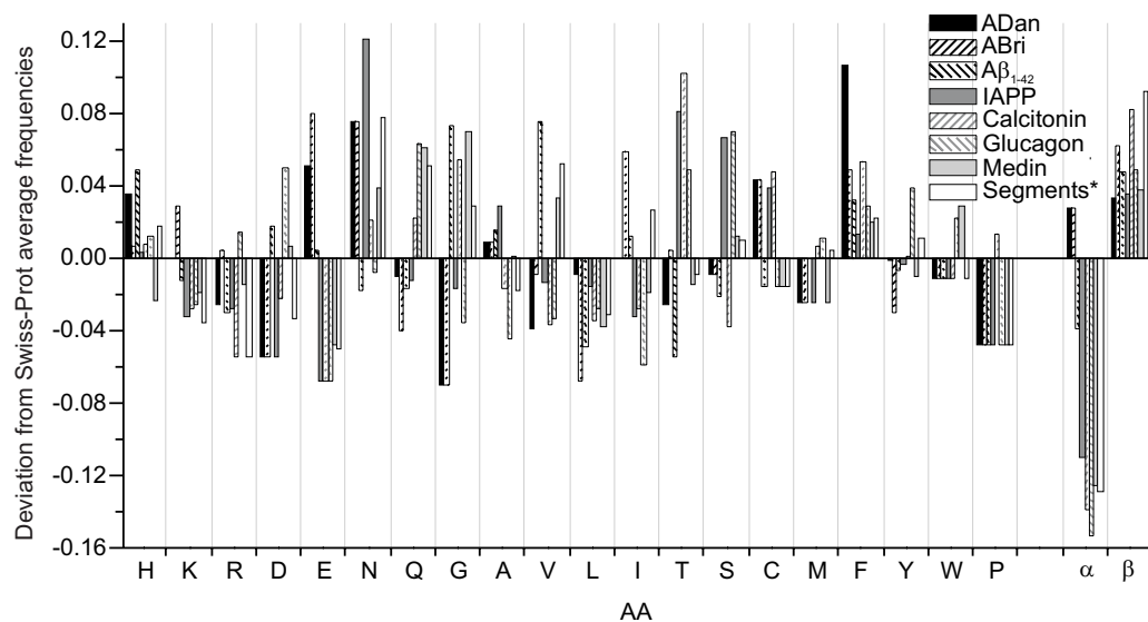
Figure 13. Deviation from the average Swiss-Prot amino acid composition ( www.expasy.ch/sprot/relnotes/relstat.html ) of small amyloidogenic peptides. *Small peptide segments examined by Eisenberg and co-workers [235].
