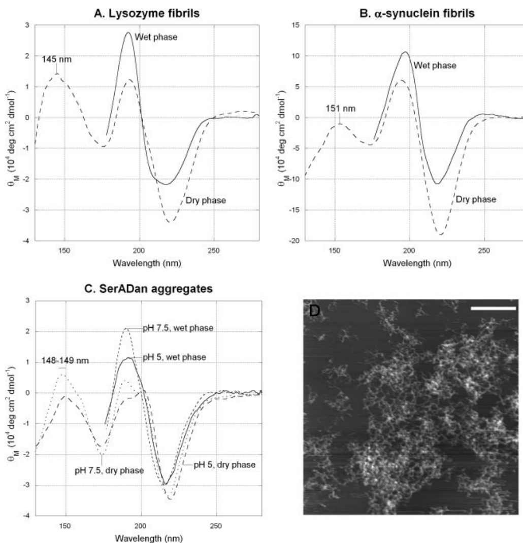
FIGURE 9 A–C. Dry phase CD spectra for fibril and aggregate samples. D. AFM of SerADan aggregates formed at pH 7.5, white bar is 1 mm.
