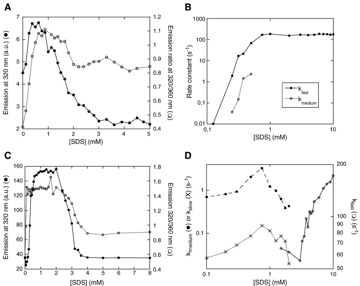
Fig. 6. Equilibrium titration of 2 \mu M S6 with SDS in 20 mM sodium acetate at (A) pH 5.5 and (C) pH 4. Kinetics of unfolding as a function of SDS concentration in 20 mM sodium acetate at (B) pH 5.5 and (D) pH 4.
