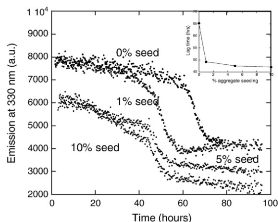
Fig. 9. Plate-reader assay of the seeding of IA8 S6 in 1.5 mM SDS using 1–10% IA8 aggregate from a previous aggregation reaction in 20 mM sodium acetate pH 5.5 at 42 °C. Insert : Lag time of fibrillation as a function of aggregate concentration.
