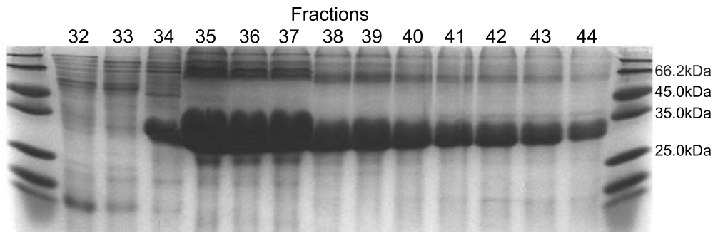
Figure 55. AEC-purified BriPP.
