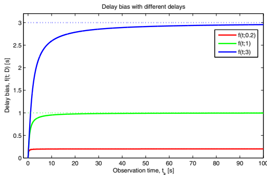
Fig. 4. Plot of the bias function f(t; D) = t(1 - \exp(-D_k/t)) for f(t; 0.2) , f(t; 1) , f(t; 3)
