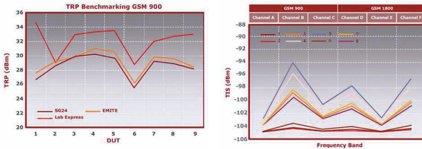
Figure 2: TRP (left) and TIS (right) benchmarking.
