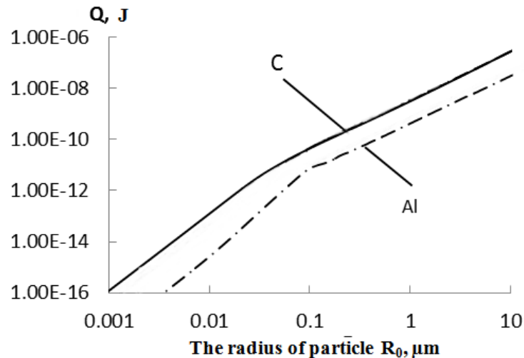
Figure 4. The heat storage near the aluminum particle (dotted line) and carbon particle (solid curve) depending on radius R_0 at energy density of the laser pulse up to 100 \text{ mJ/cm}^2 for the wavelength \lambda_0=1064 \text{ nm} .
