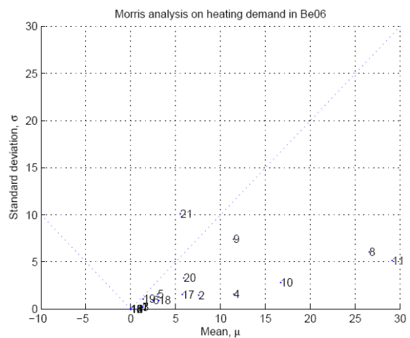
Figure 4. Influence of design parameters on the heating demand.
