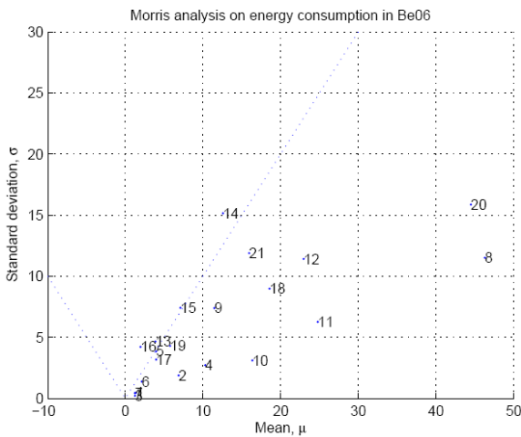
Figure 3. Influence of design parameters on the total energy use.
